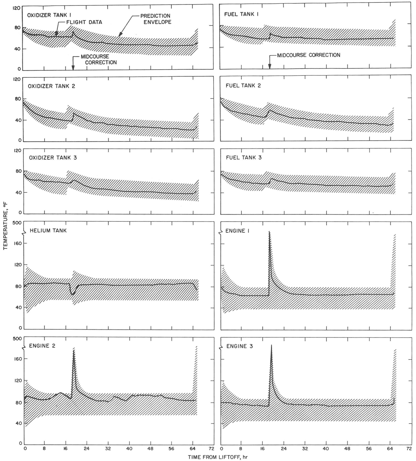
Fig. D-4. Vernier propulsion system transit temperatures
