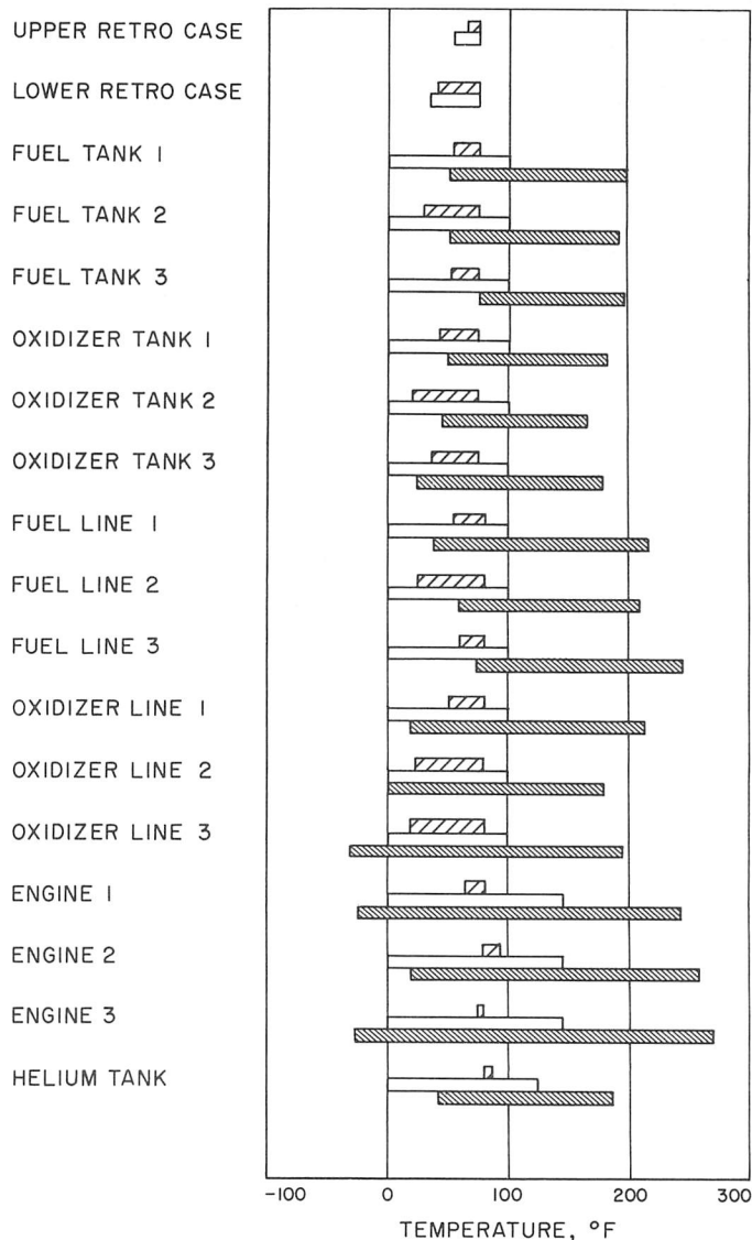
Fig. IV-27. Propulsion system temperature ranges during transit and lunar day
