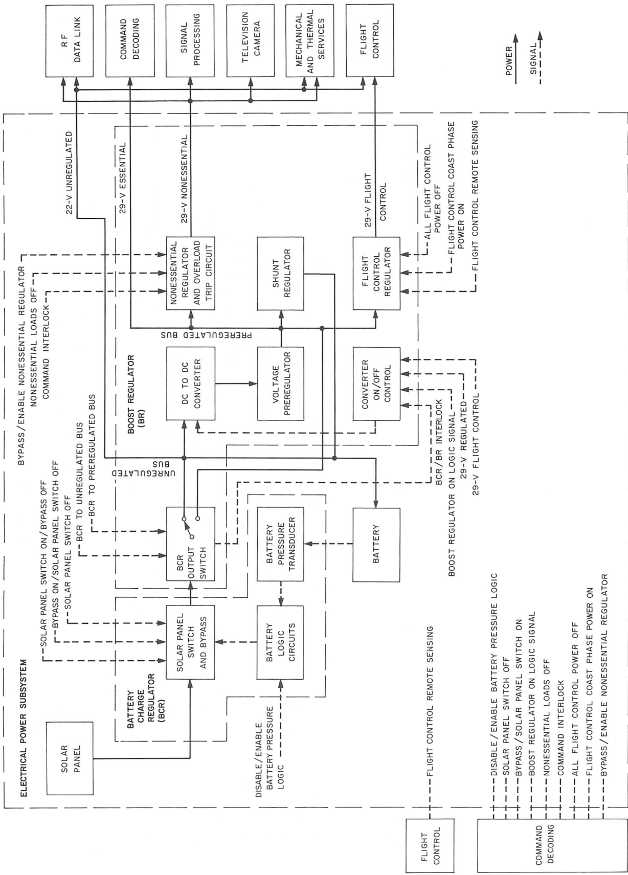
Fig. IV-18. Functional diagram of Surveyor VI electrical power subsystem
