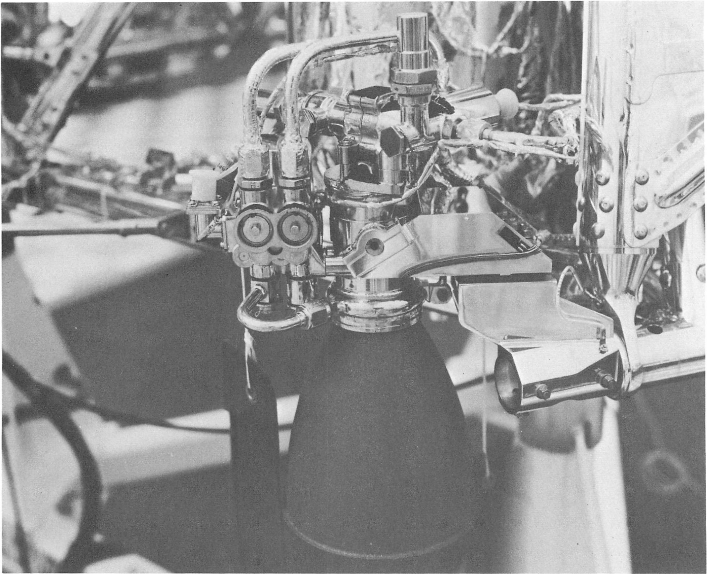
Fig. IV-26. Vernier engine thrust chamber assembly
