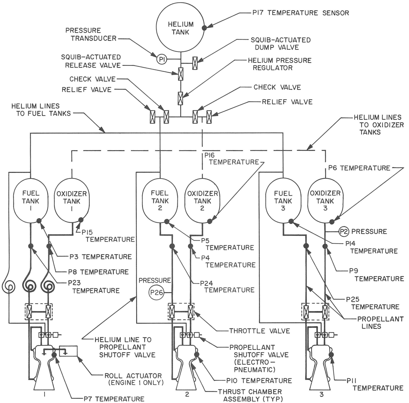
Fig. IV-23. Vernier propulsion system schematic
