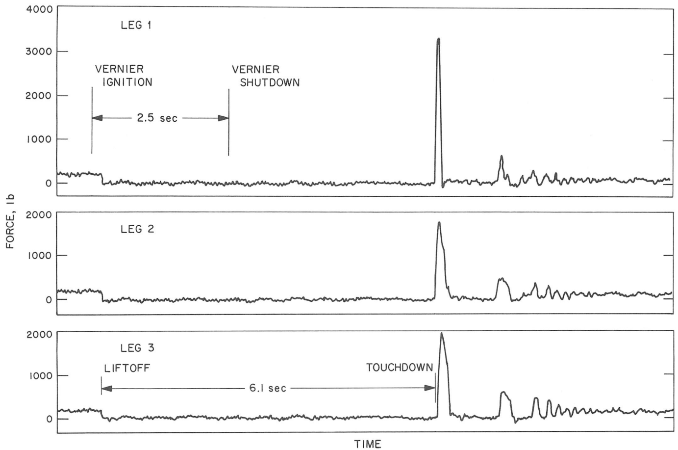
Fig. IV-14. Loads on shock absorbers during spacecraft hop experiment landing
