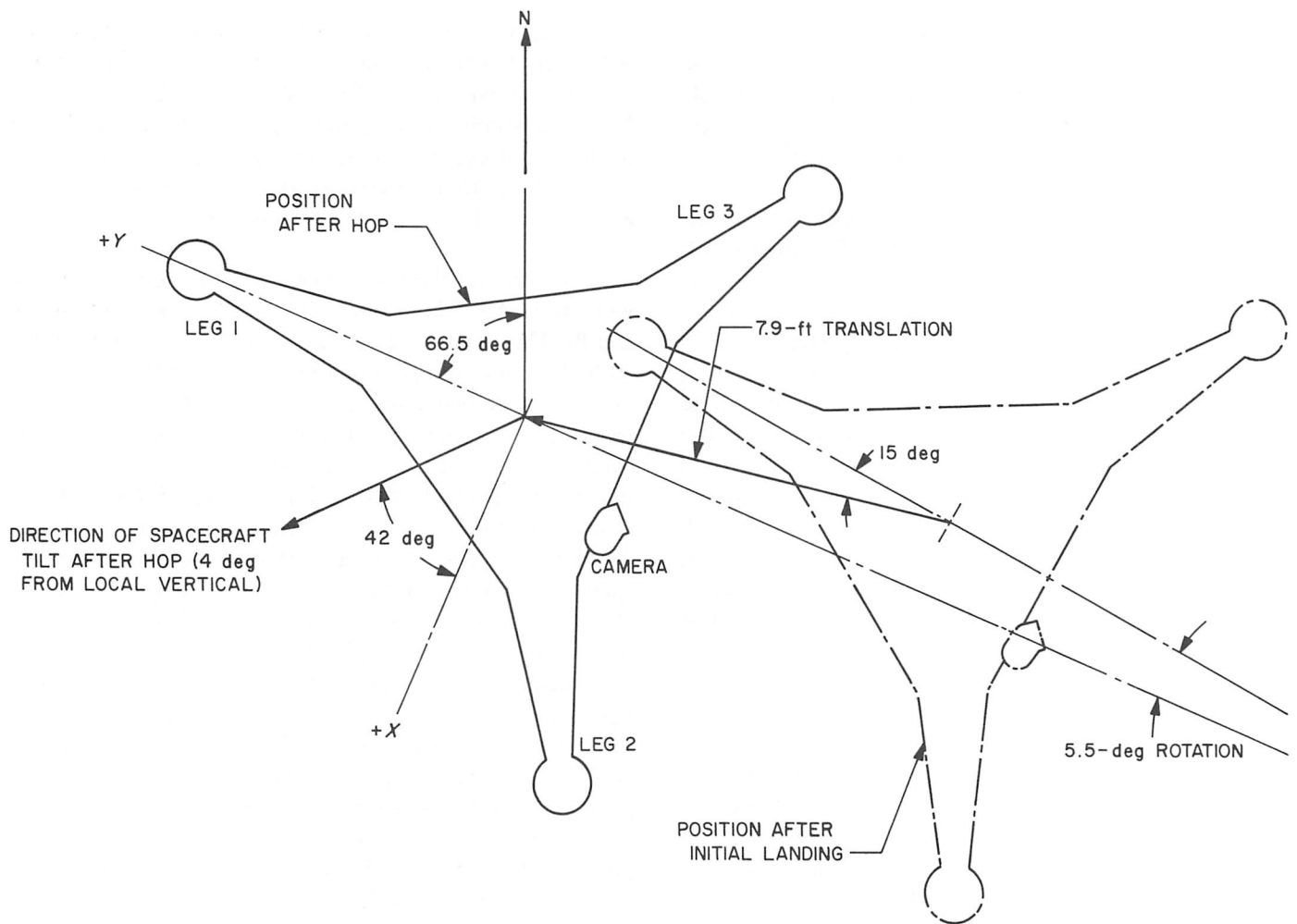
Fig. IV-10. Change in spacecraft position resulting from hop
