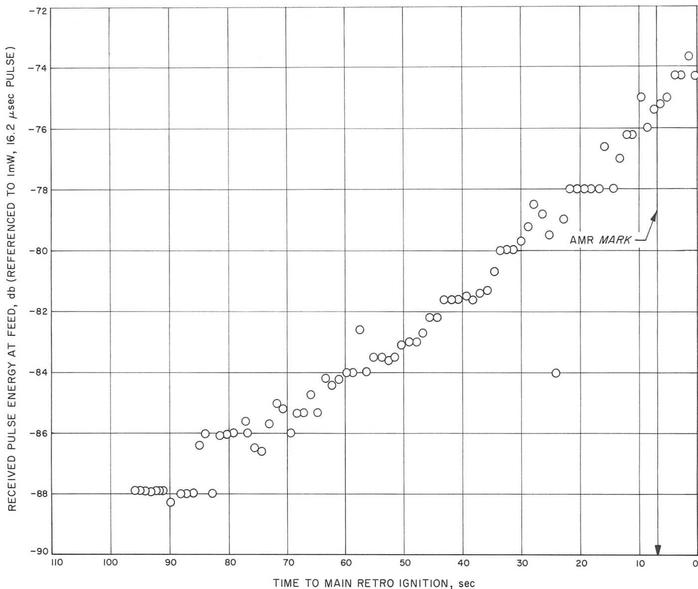
Fig. IV-37. Altitude marking radar AGC
