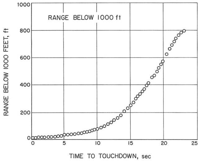
Fig. IV-44. Slant range vs time during terminal descent
