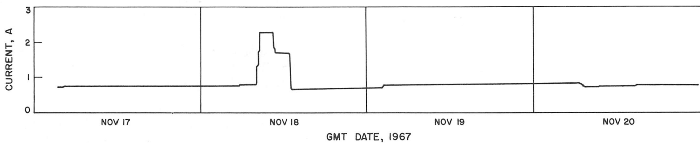
Fig. IV-20. Typical postlanding regulated current requirements
