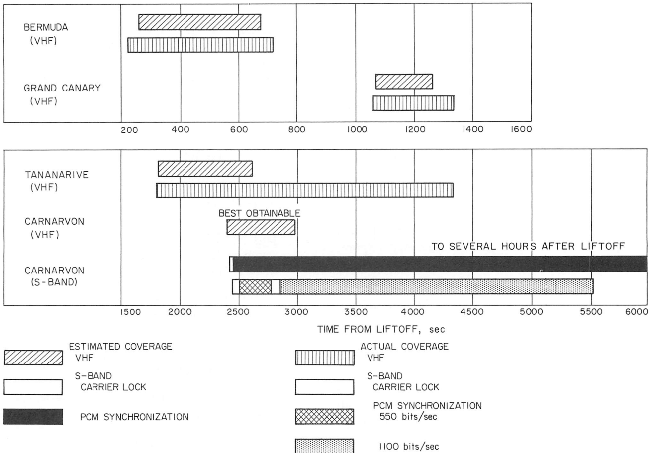
Fig. V-6. MSFN VHF and S-band telemetry coverage
