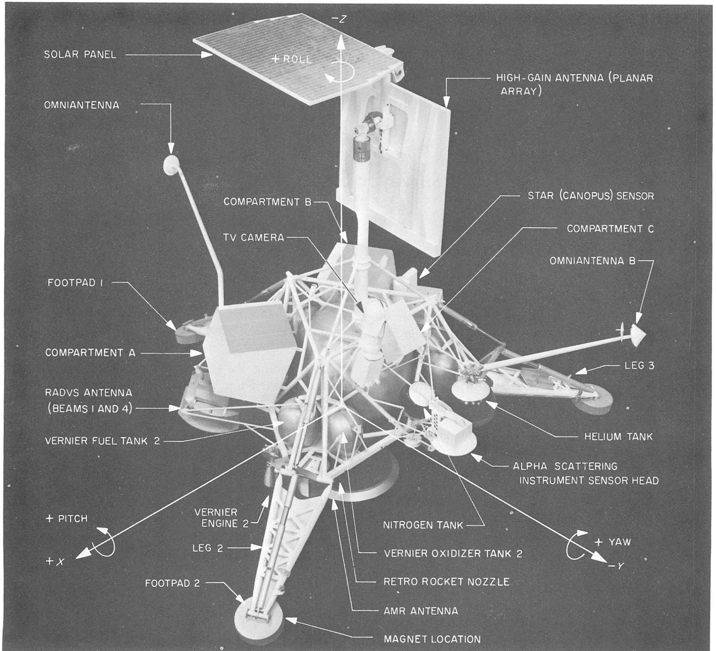
Fig. IV-1. Surveyor VI spacecraft in cruise mode
