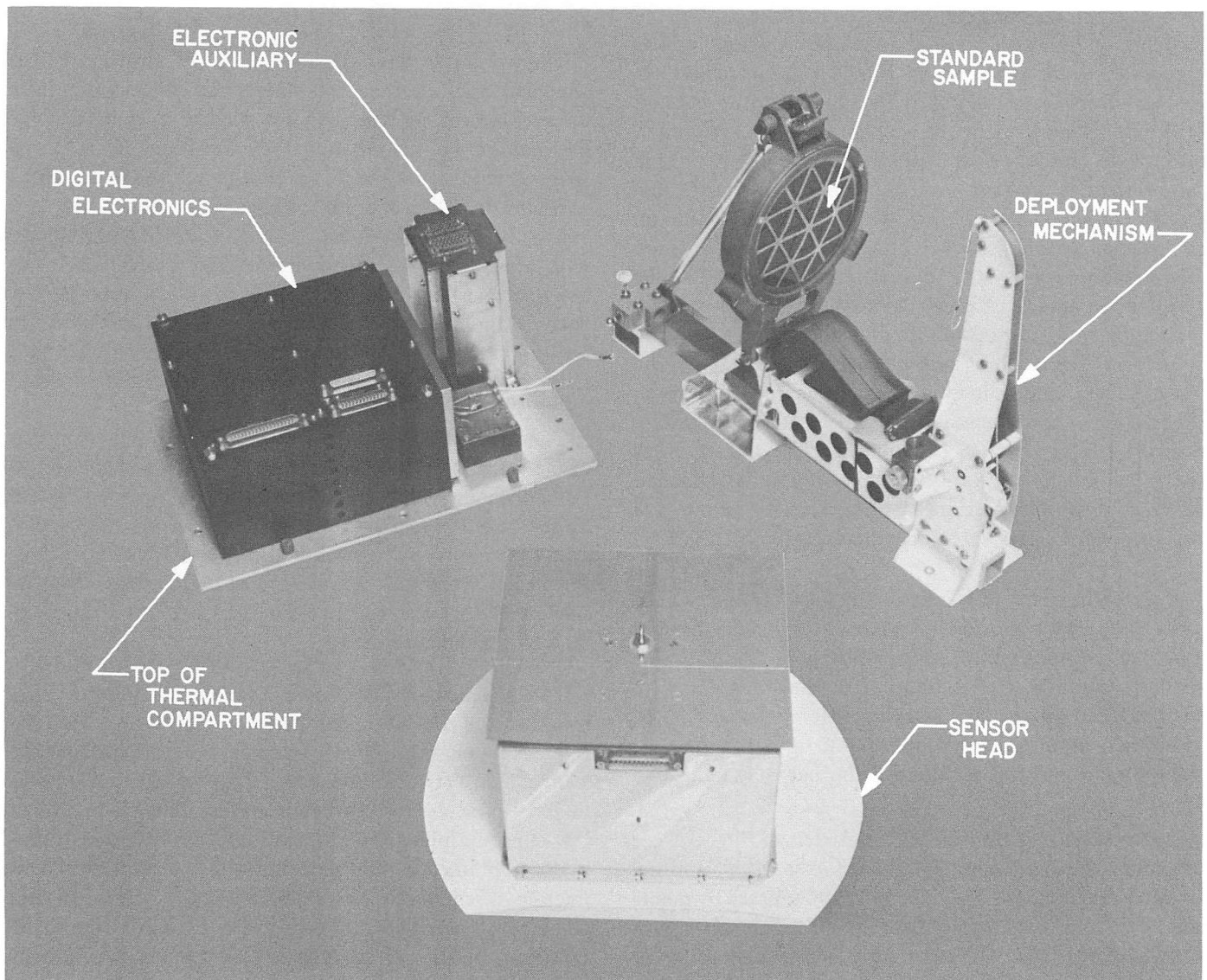
Fig. IV-56. Alpha scattering instrument components
