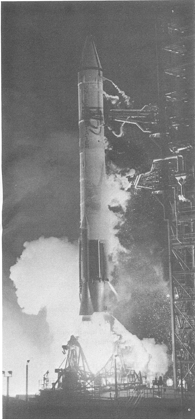
Fig. II-3. Atlas/Centaur AC-14 launching Surveyor VI
