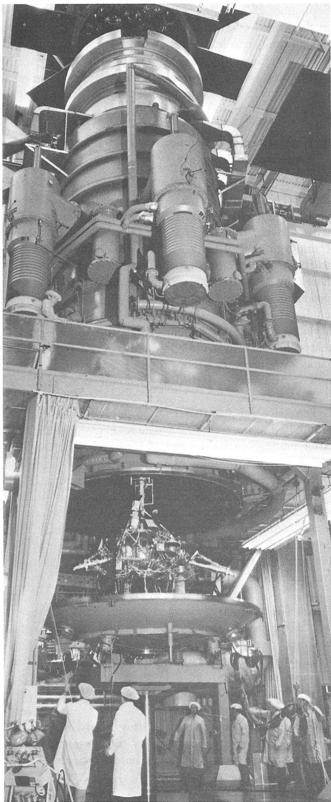
Fig. II-1. Removal of Surveyor VI spacecraft from solar-thermal-vacuum chamber after initial tests
