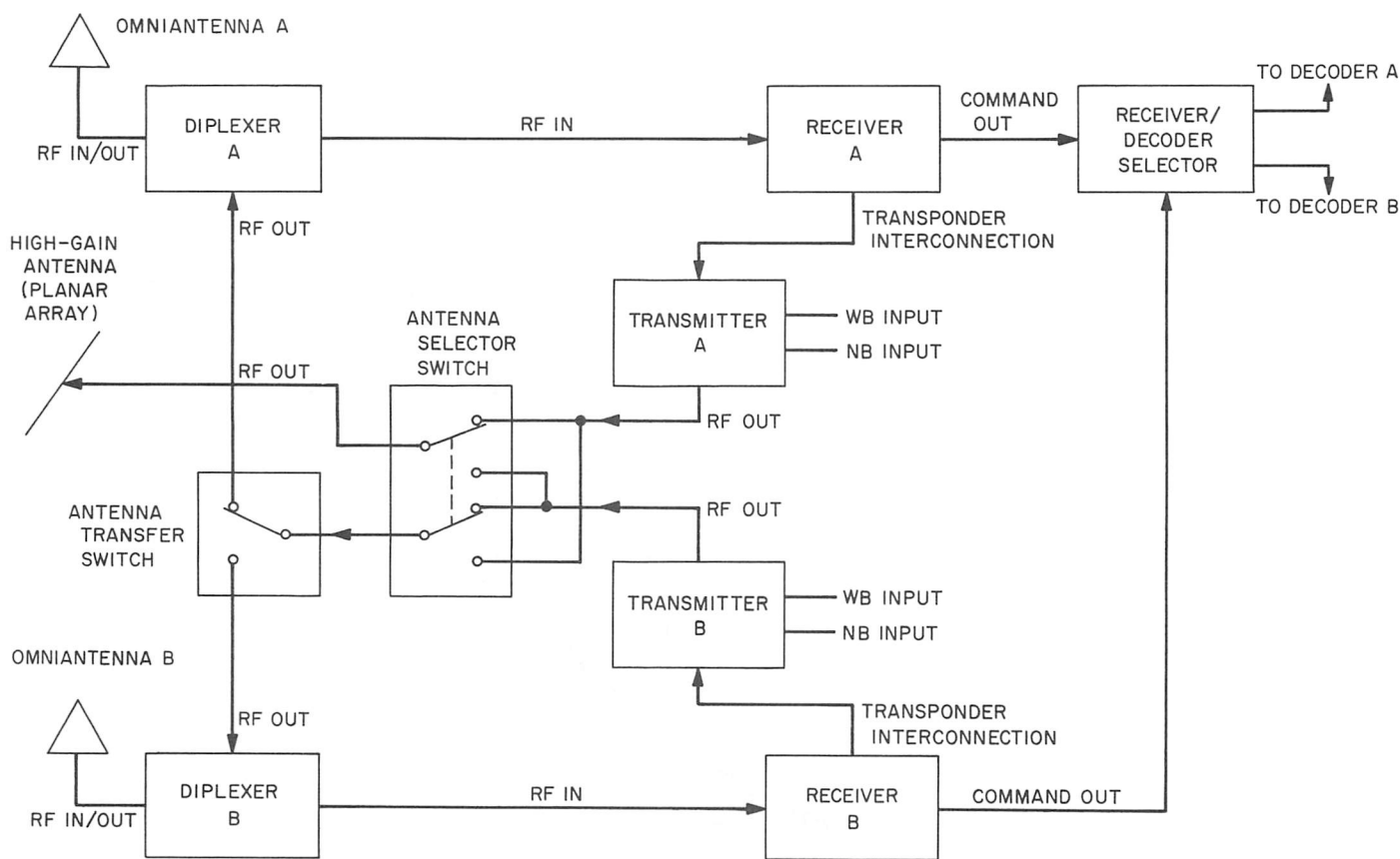
Fig. IV-45. Radio subsystem block diagram
