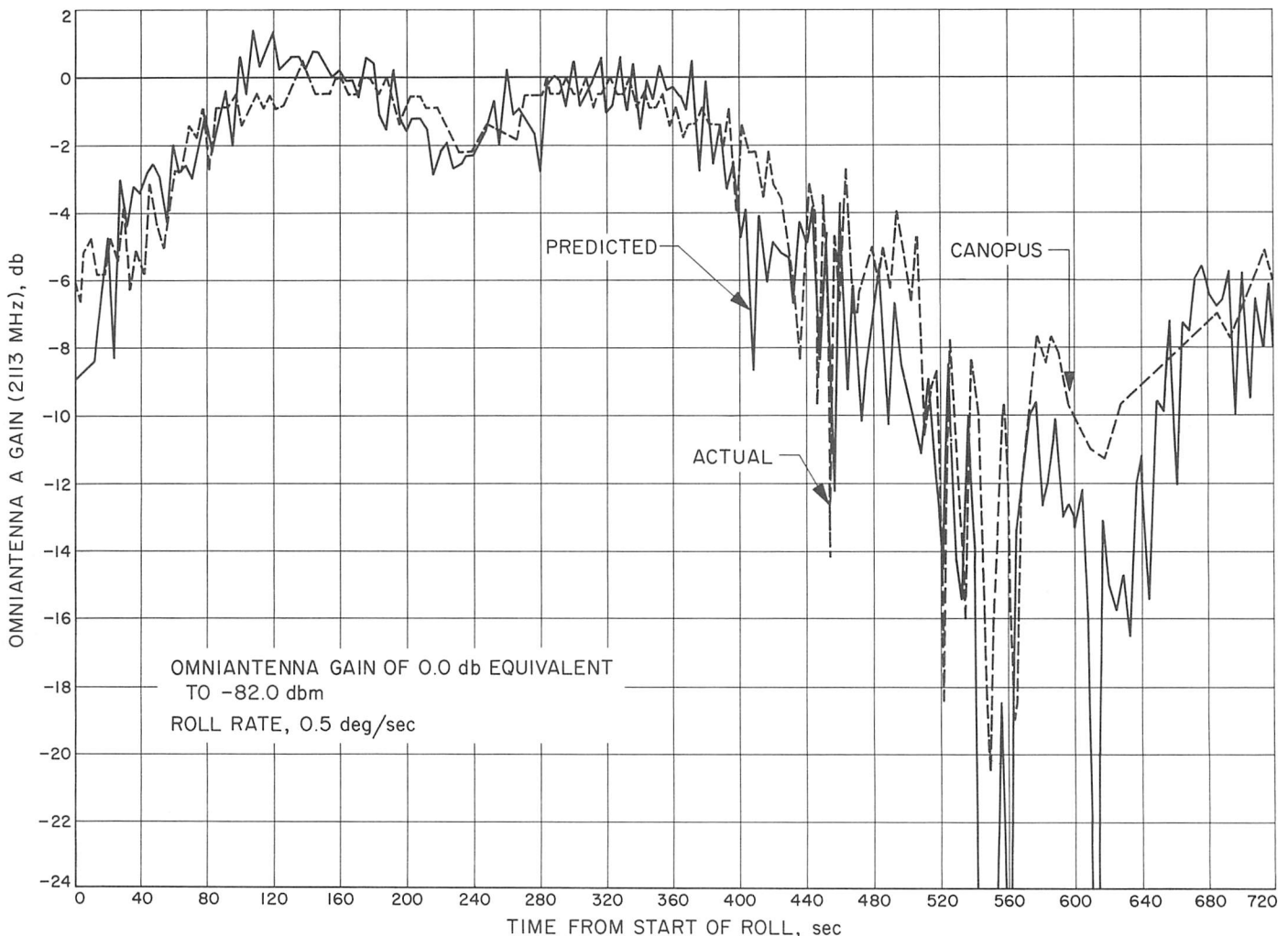
Fig. IV-46. Spacecraft Receiver A signal level during star verification/acquisition roll
