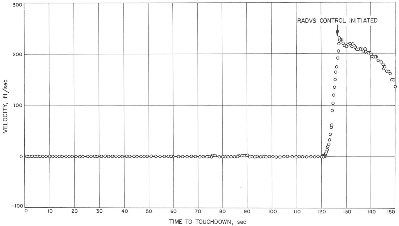
Fig. IV-42. Y-component of velocity V_y during descent
