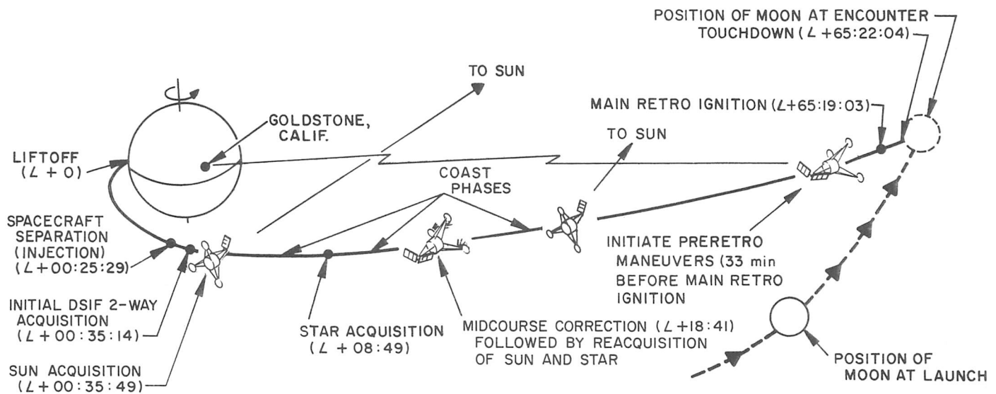
Fig. 1-1. Transit phase major events
