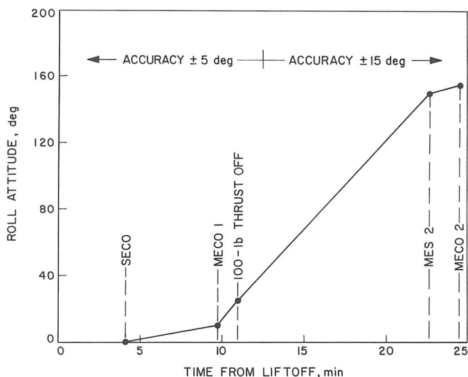
Fig. III-4. Centaur clockwise roll attitude relative to local vertical
