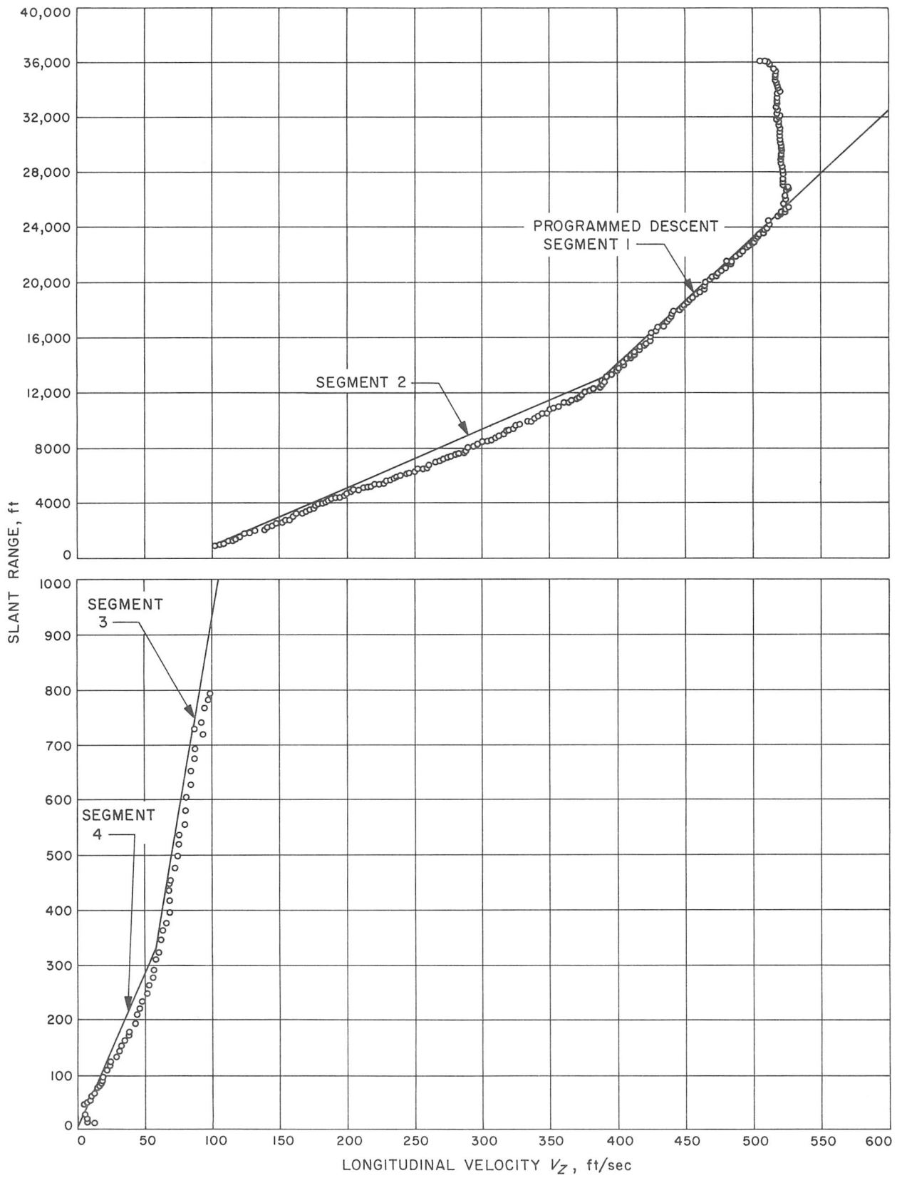
Fig. IV-8. Surveyor VI descent profile
