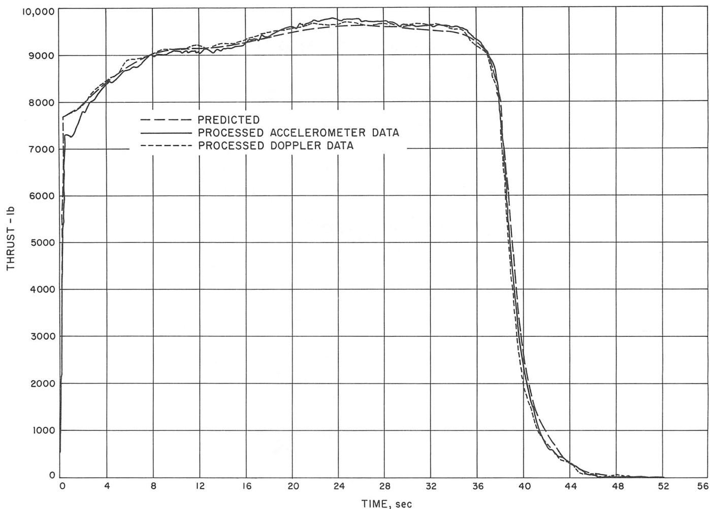
Fig. IV-33. Surveyor VI main retromotor thrust vs time
