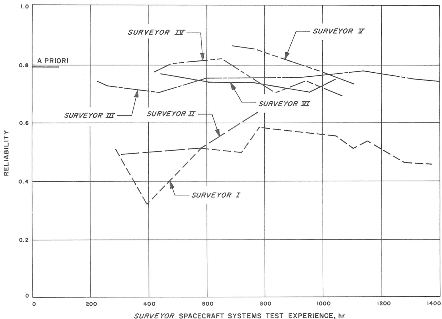
Fig. IV-4. Surveyor spacecraft system reliability estimates
