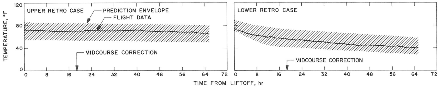
Fig. D-5. Main retromotor transit temperatures
