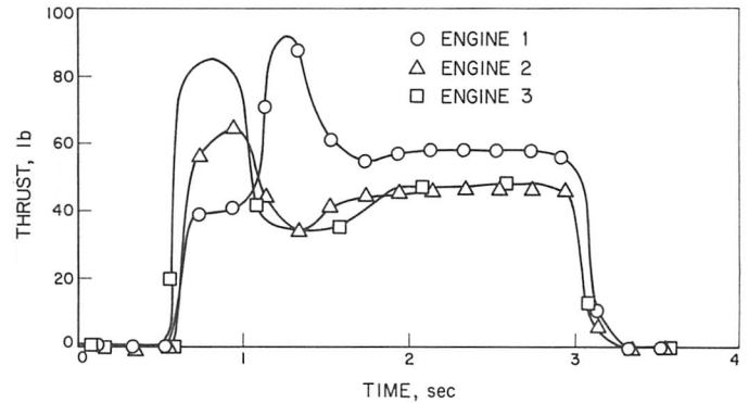
Fig. IV-29. Vernier engine thrust values during spacecraft hop experiment
