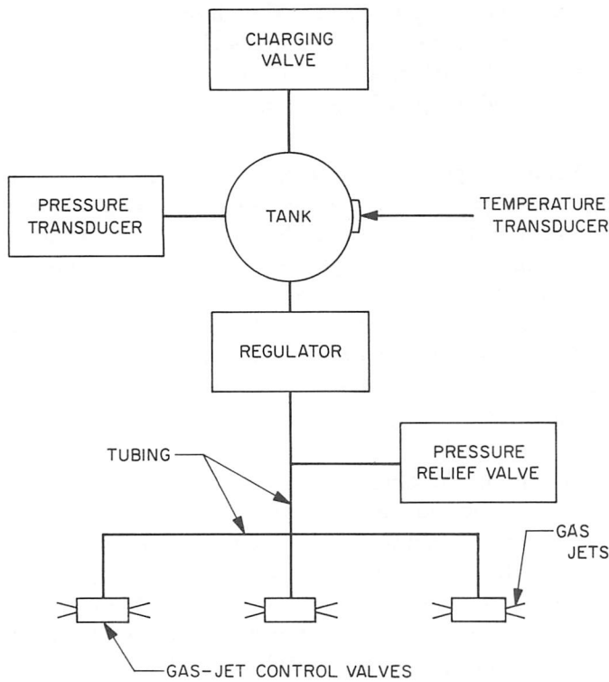
Fig. IV-35. Gas-jet attitude control system
