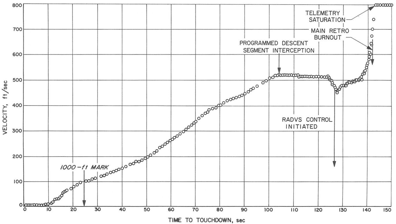
Fig. IV-43. Z-component of velocity V_z during descent
