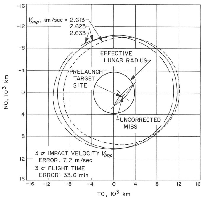
Fig. VII-5. Midcourse correction capability contours (for a correction 20 hr after injection)
