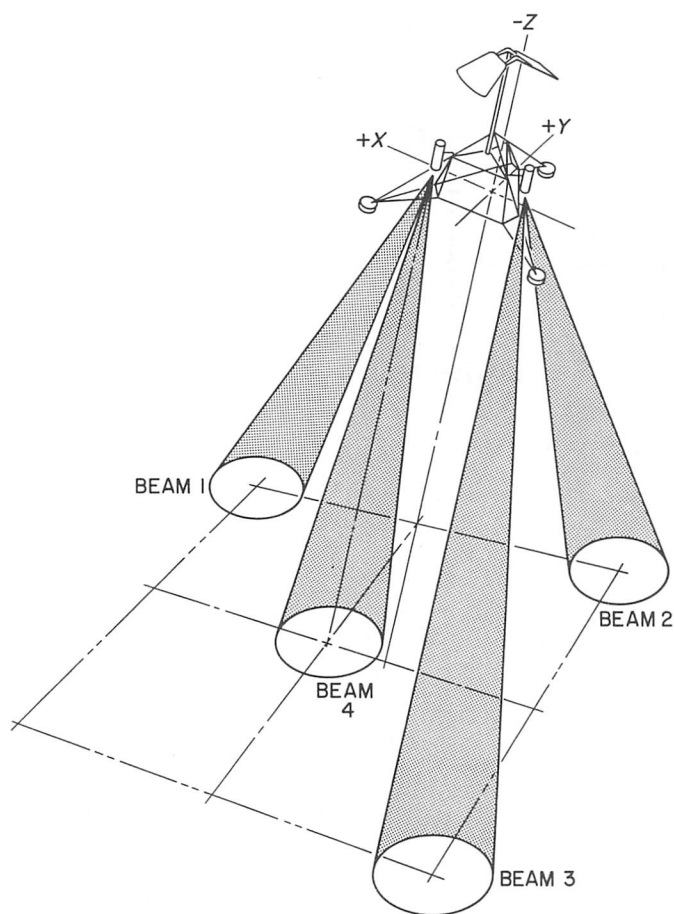
Fig. IV-39. RADVS beam orientation
