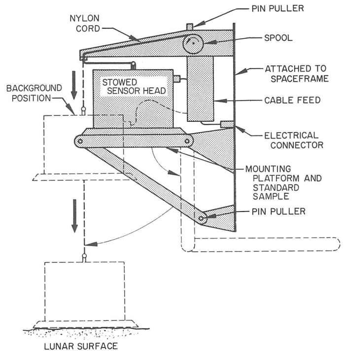
Fig. IV-59. Alpha scattering instrument deployment mechanism
