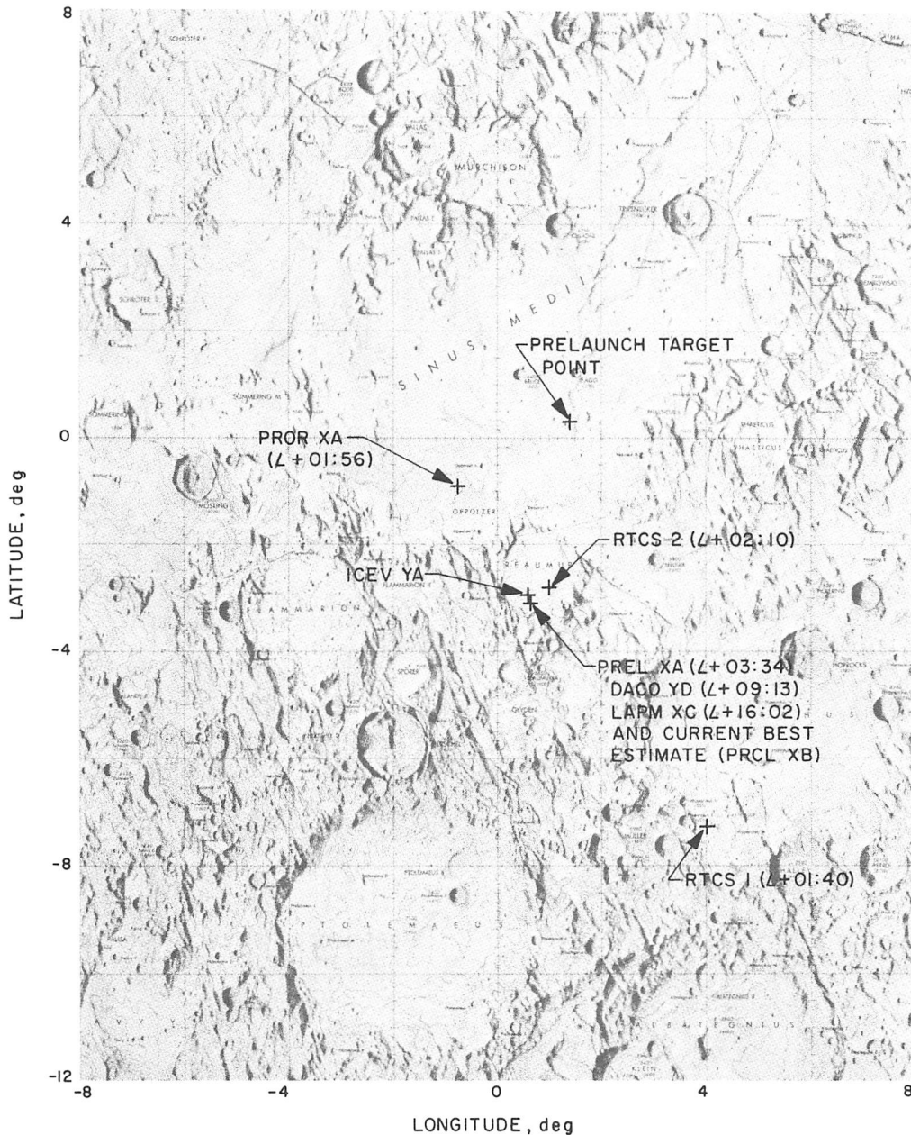
Fig. VII-3. Surveyor VI pre-midcourse unbraked impact locations
