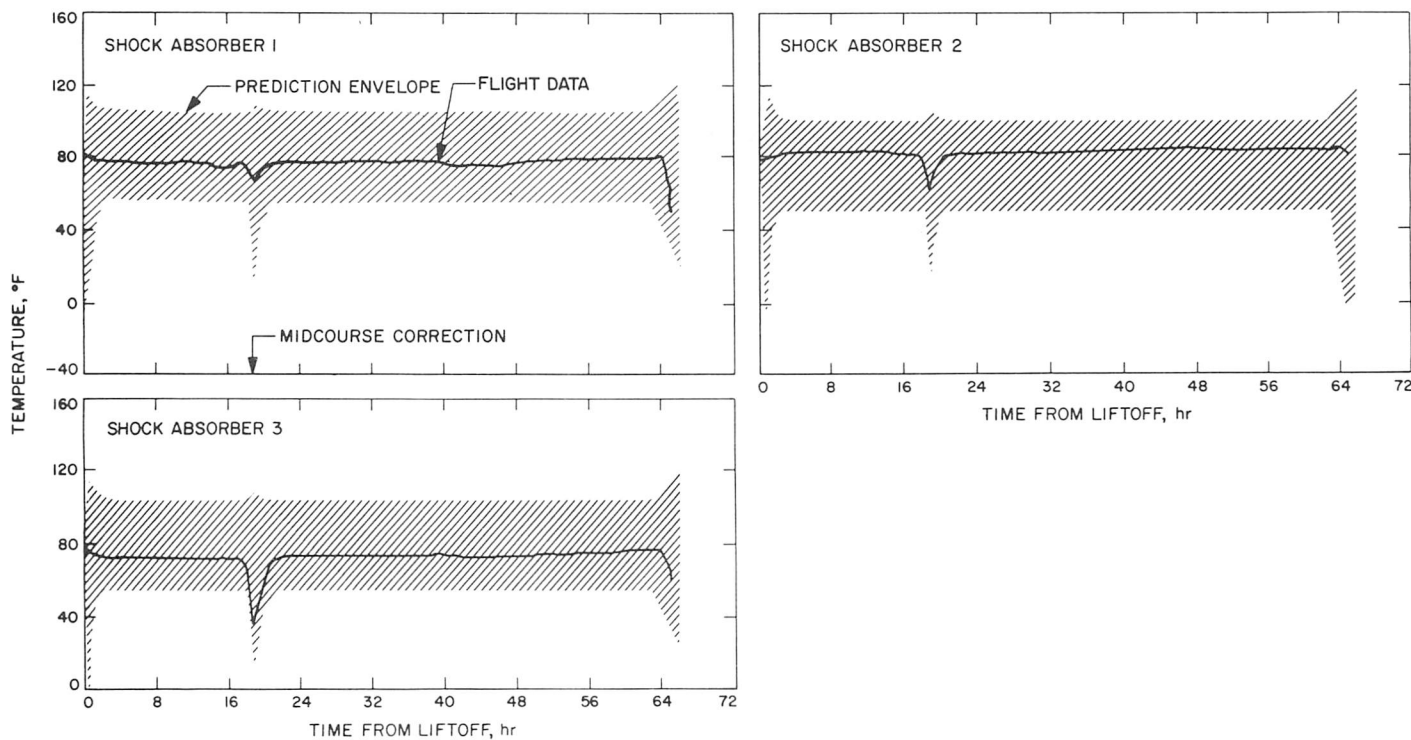
Fig. D-1. Landing gear transit temperatures
