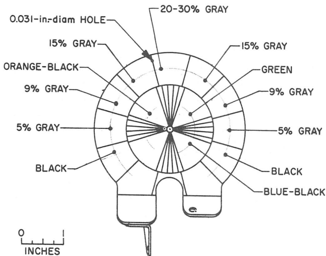
Fig. IV-55. TV photometric/colorimetric reference chart
