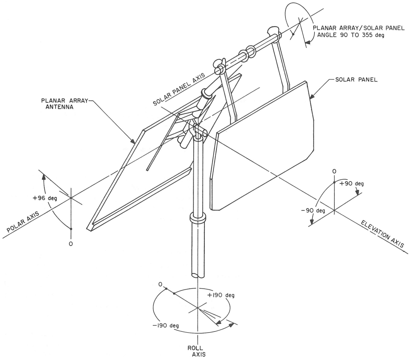
Fig. IV-15. Antenna/solar panel configuration
