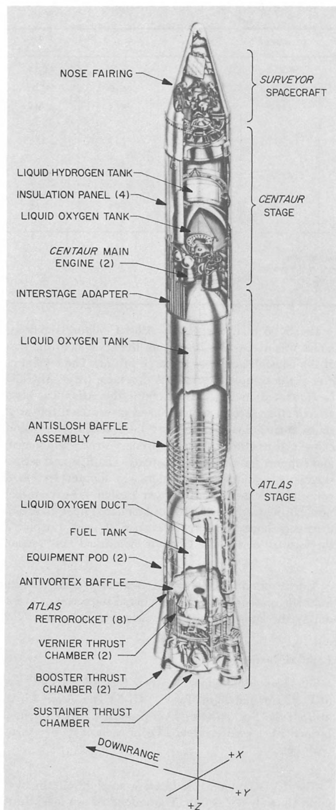
Fig. VIII-2. Atlas (SLV-3C)/Centaur/Surveyor space vehicle configuration
