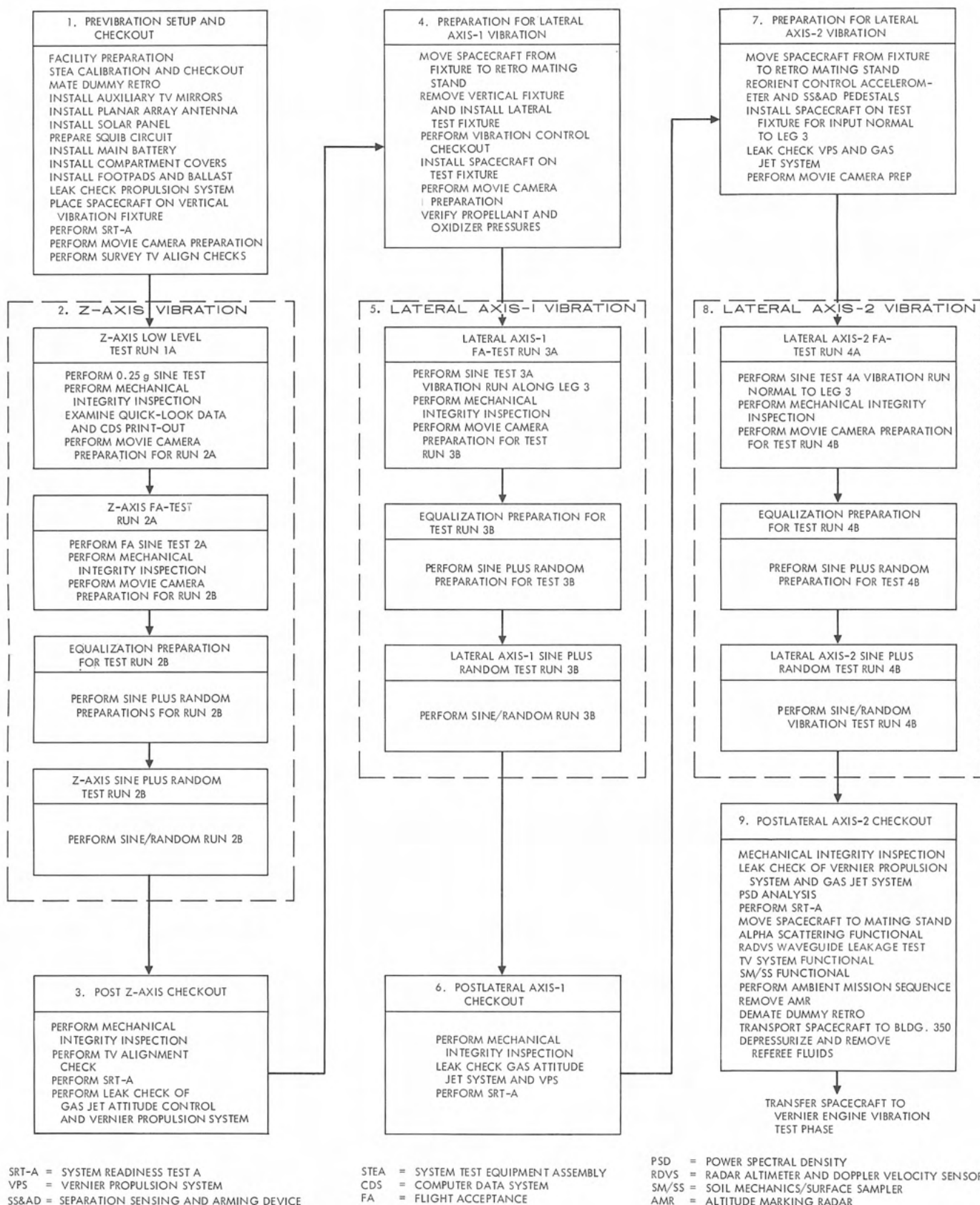
Fig. XI-13. Vibration test phase flow diagram
