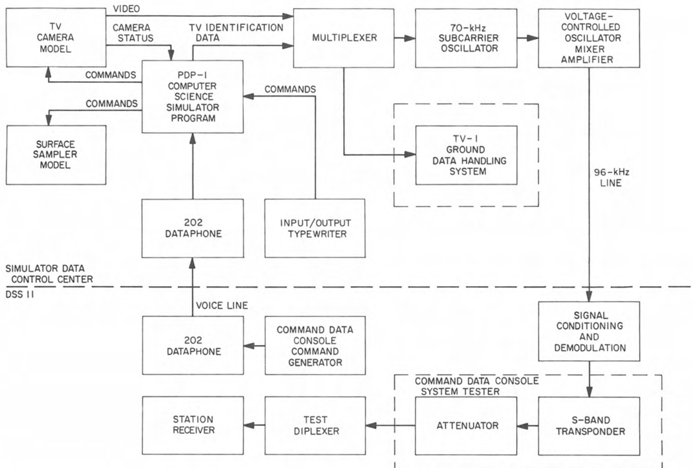
Fig. VII-14. Television/surface sampler simulation system configuration
