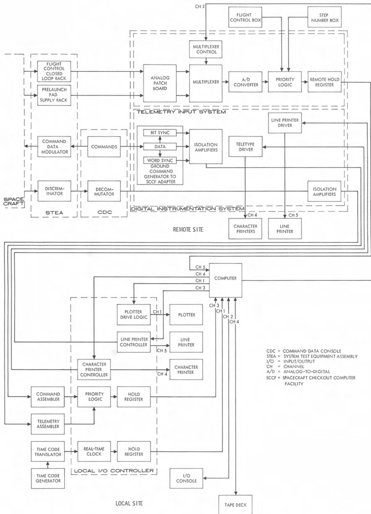
Fig. XI-3. Spacecraft checkout functional block diagram
