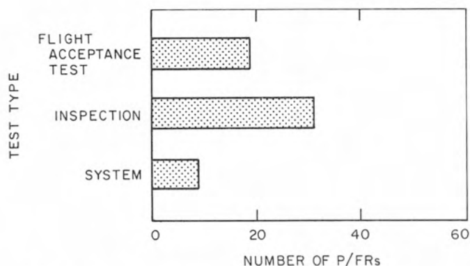
Fig. XII-21. Surveyor vernier engine problem/failure reports by test type
