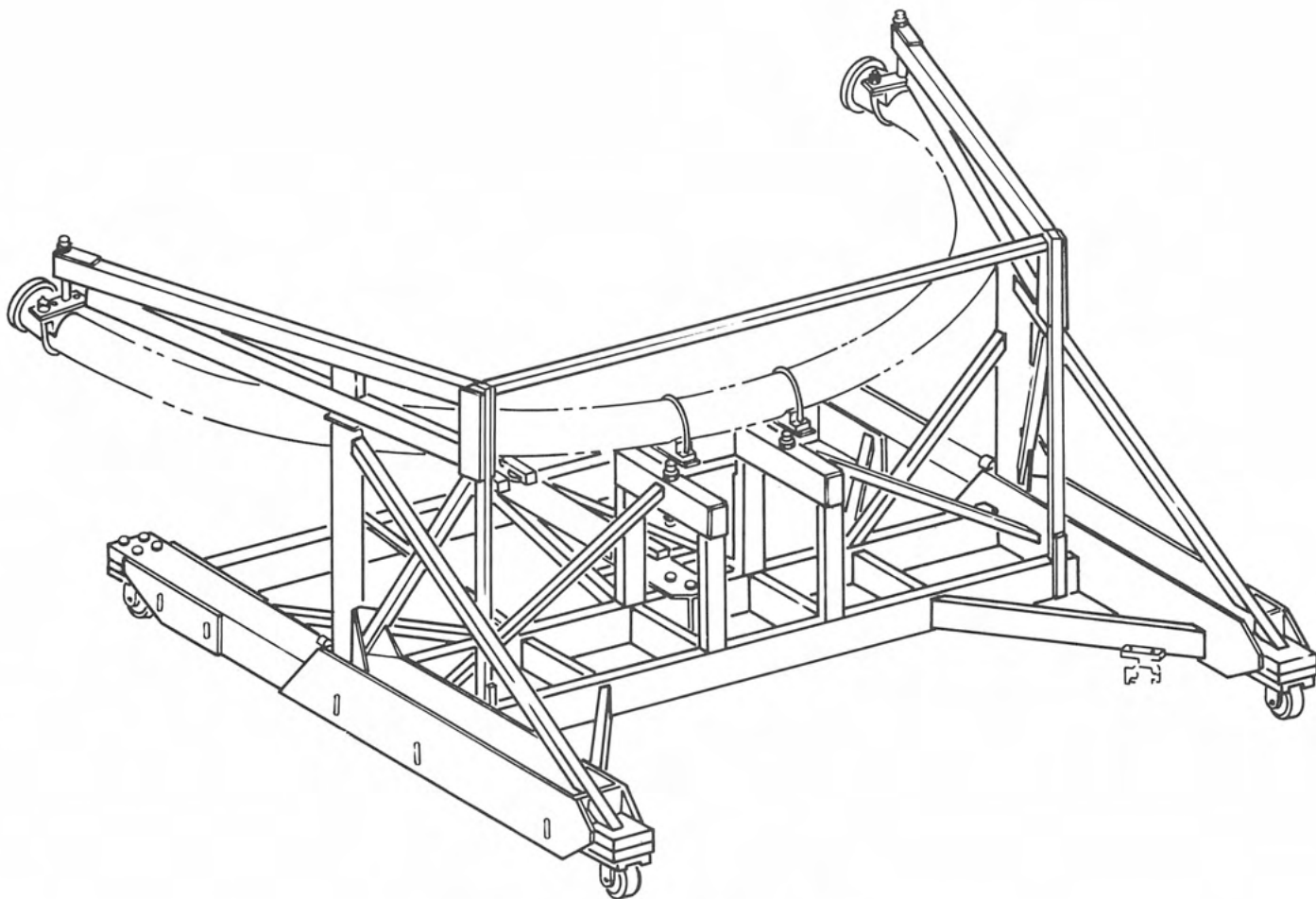
Fig. VIII-28. Nose fairing handling cart
