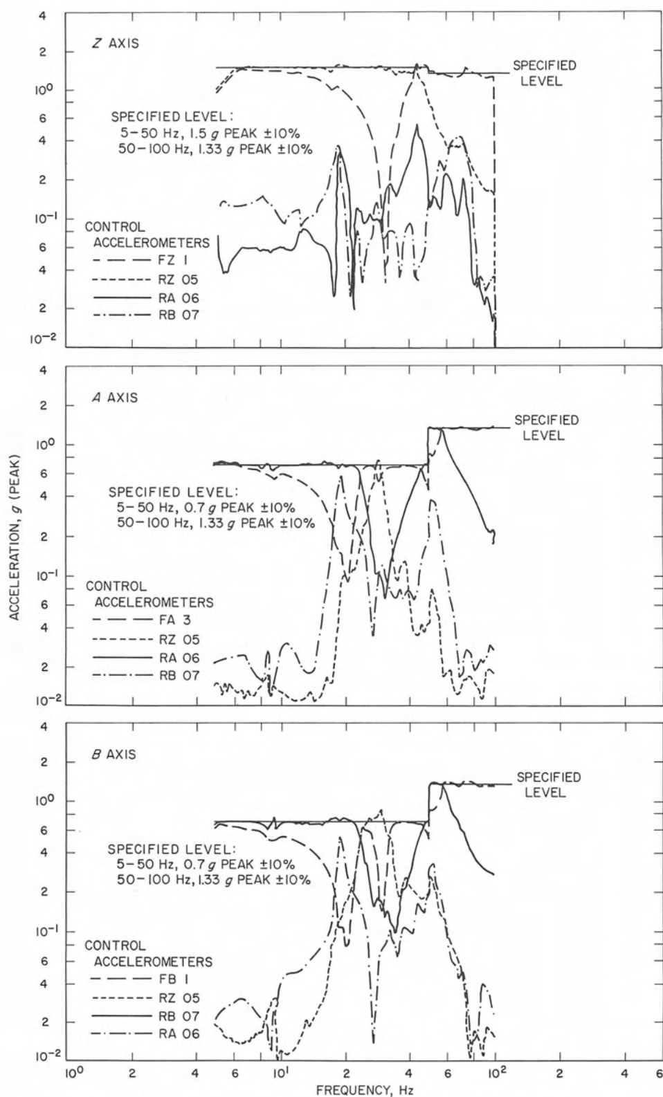
Fig. X-10. SC-7 low-frequency sinusoidal vibration input level vs specification values
