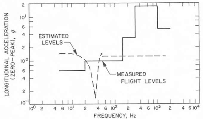
Fig. X-14. Comparison of the 95% flight equivalent sinusoidal vibration environment and the estimated sinusoidal vibration environment for the longitudinal axis
