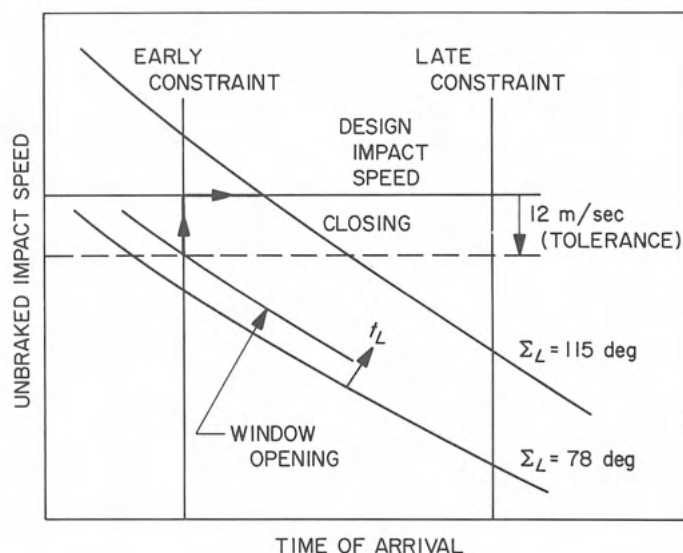
Fig. VI-16. Corner targeting
