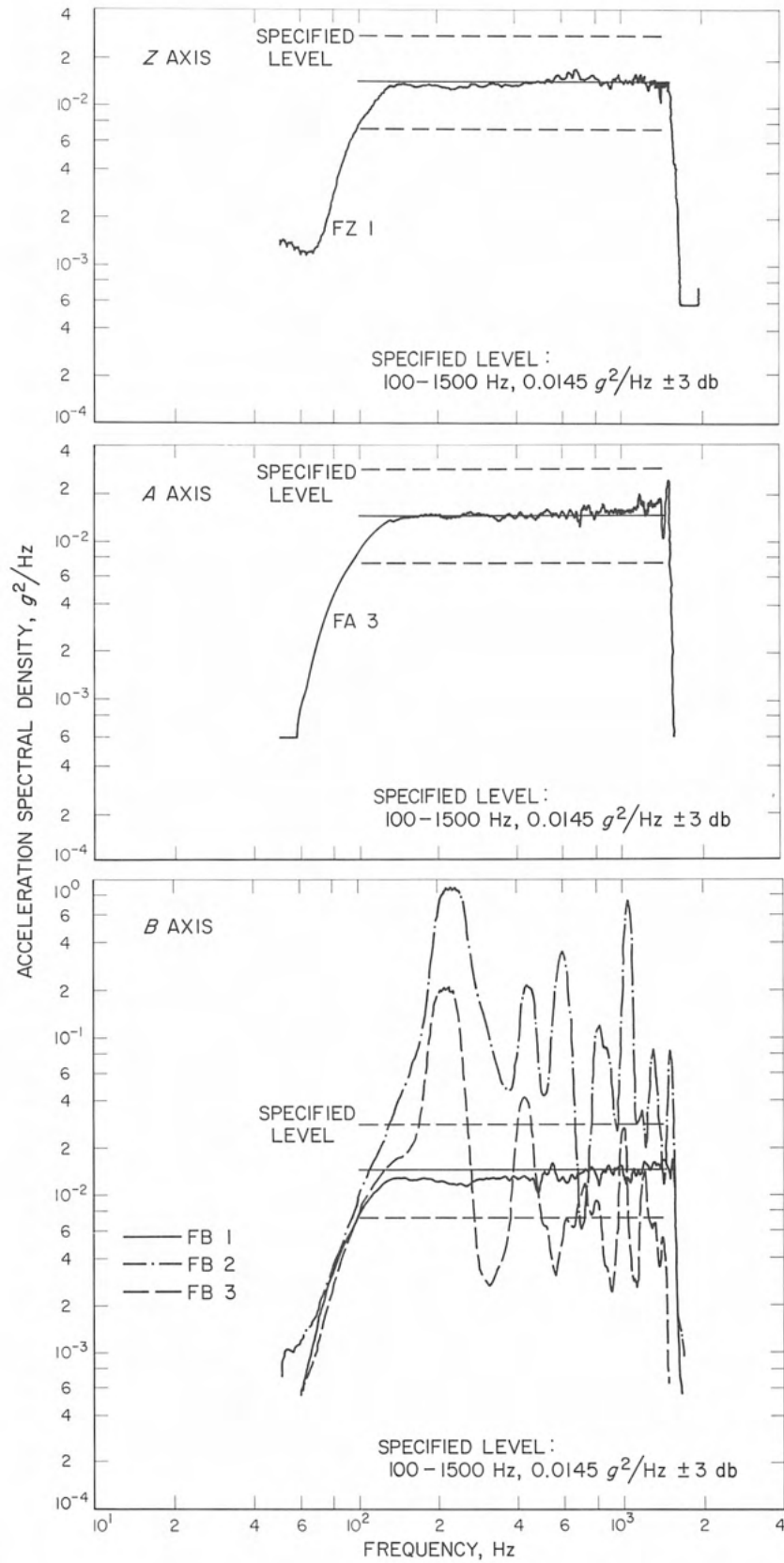
Fig. X-12. SC-3 random vibration input level vs specification values
