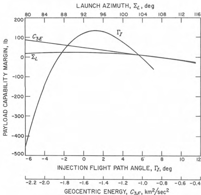
Fig. VI-7. Payload capability margin
