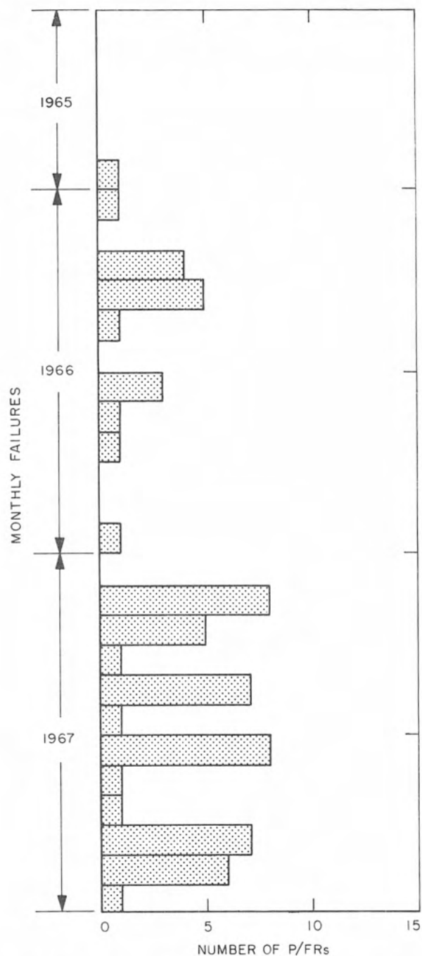
Fig. XII-23. Surveyor vernier engine problem/failure reports by month
