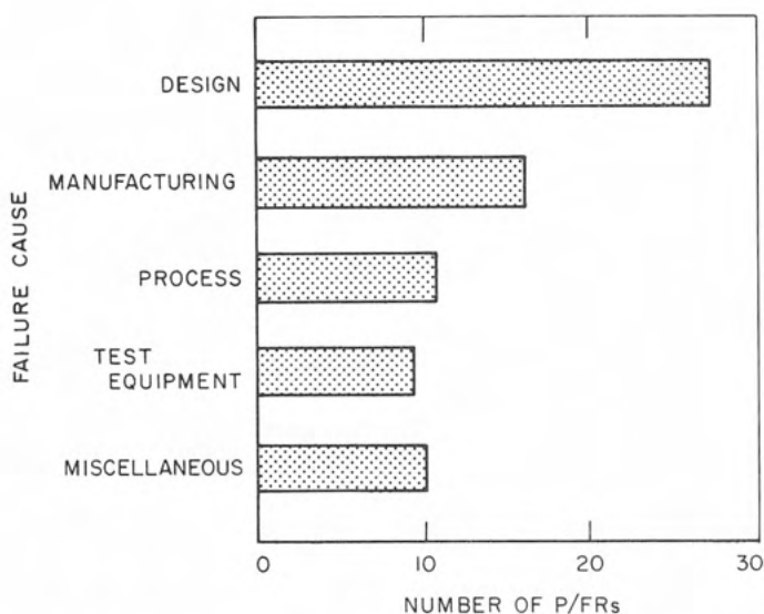
Fig. XII-22. Surveyor vernier engine problem/failure reports by failure cause
