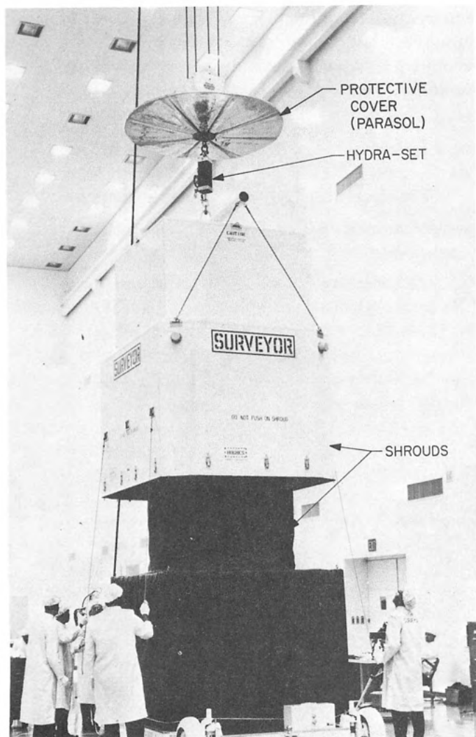
Fig. IX-2. Ground transport vehicle GTV-1
