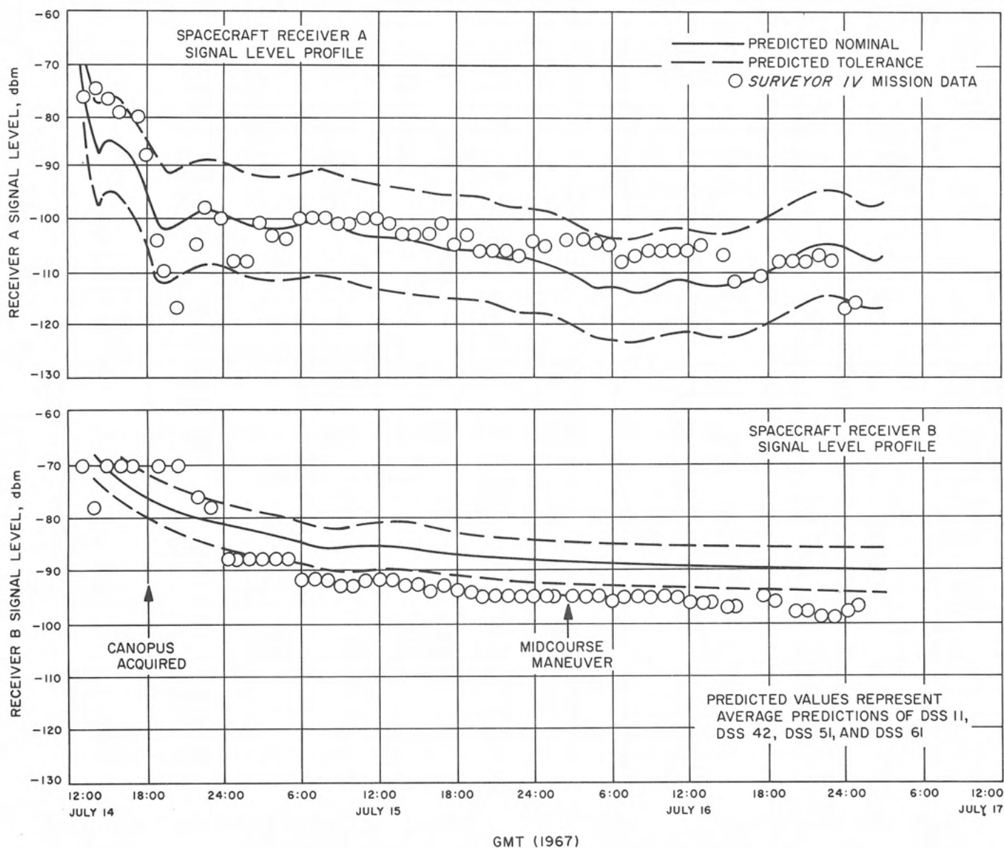
Fig. VI-36. Surveyor IV spacecraft receiver signal level profile
