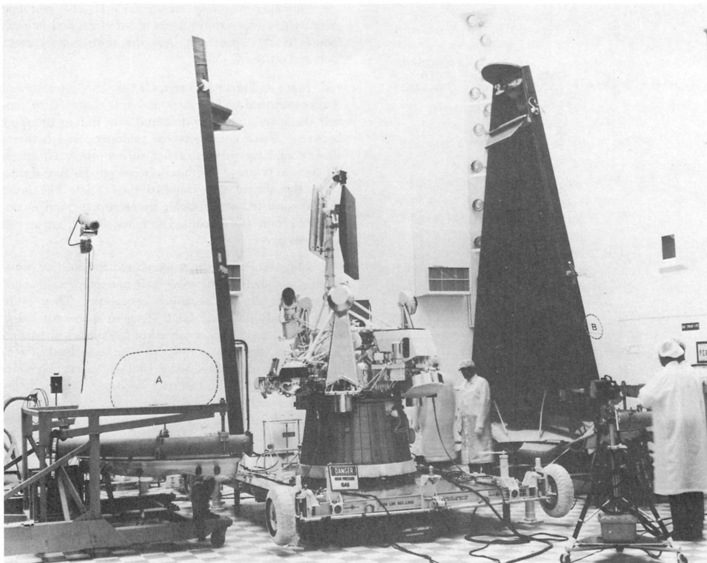
Fig. IX-3. Ground transport vehicle GTV-2
