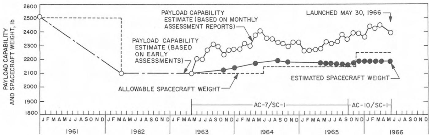
Fig. VIII-1. Atlas/Centaur payload capability history (direct-ascent— Surveyor I )
