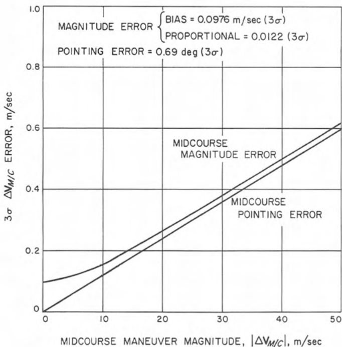
Fig. VI-24. Midcourse execution error
