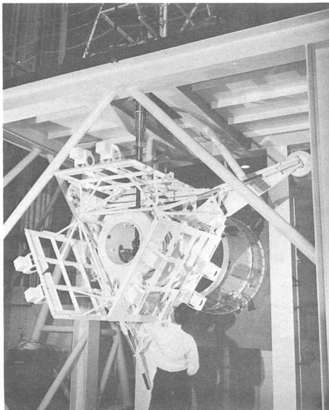
Fig. VIII-18. Spacecraft separation system test configuration
