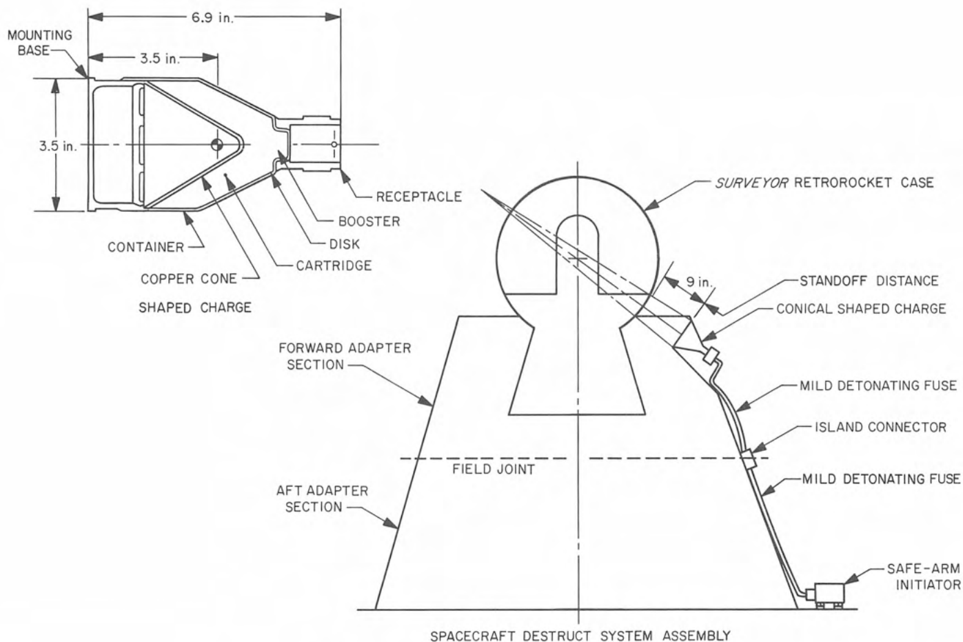
Fig. VIII-14. Spacecraft destruct system
