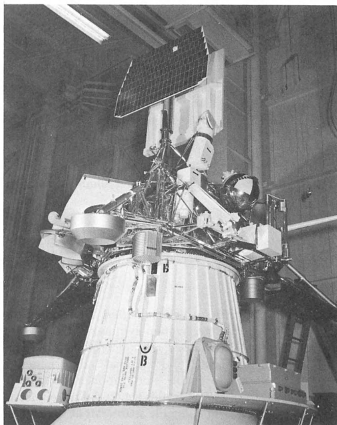
Fig. VIII-17. Spacecraft mated to Centaur
