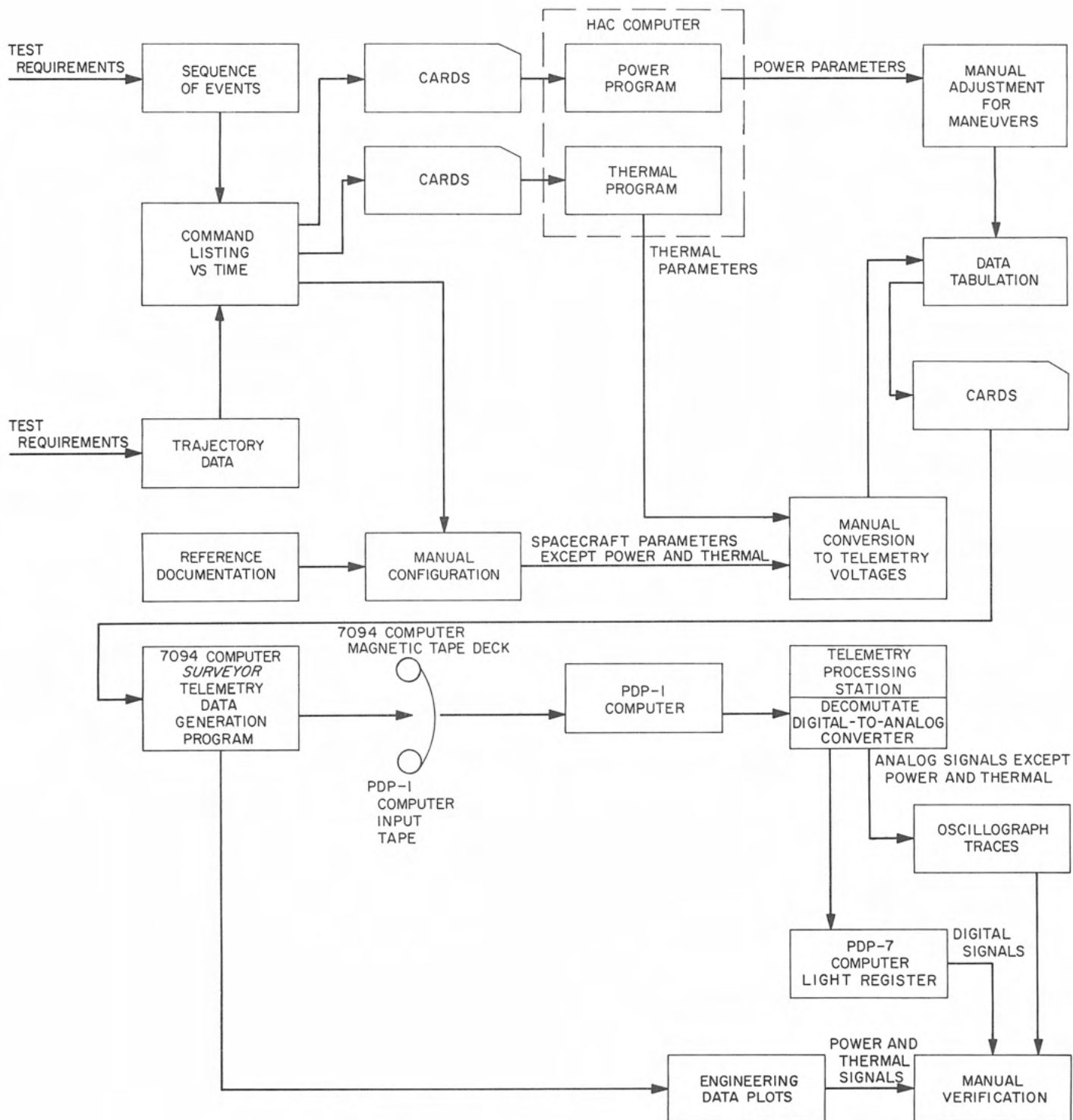
Fig. VII-12. Simulated telemetry data preparation and checkout sequence
