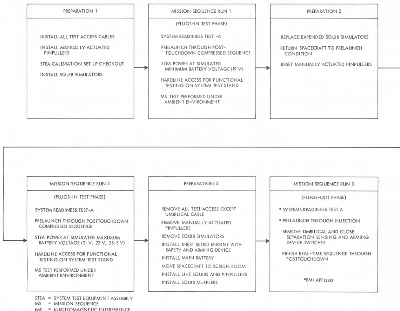
Fig. XI-8. Mission sequence/electromagnetic interference test phase flow diagram
