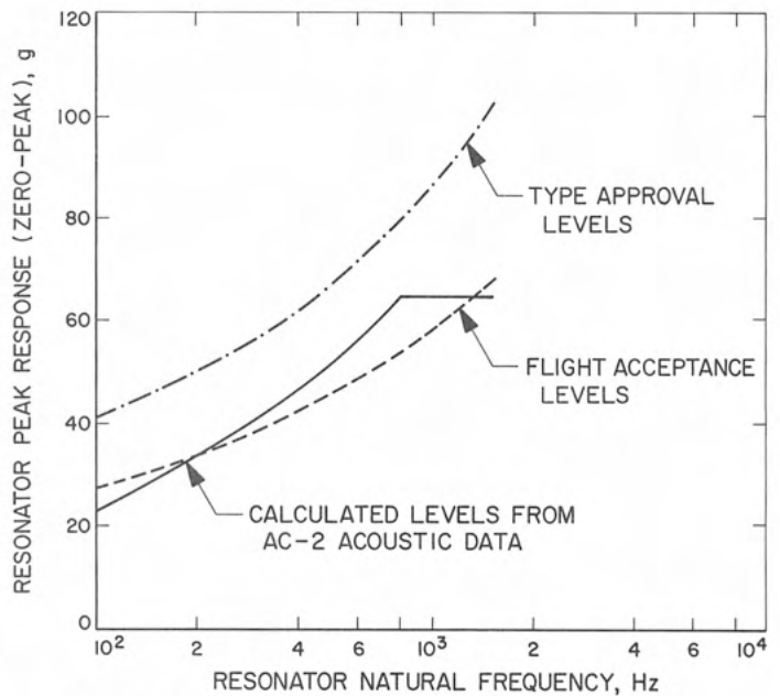
Fig. X-1. Single-degree-of-freedom resonator peak response for excitations consisting of the FA and TA combined sine-random environments
