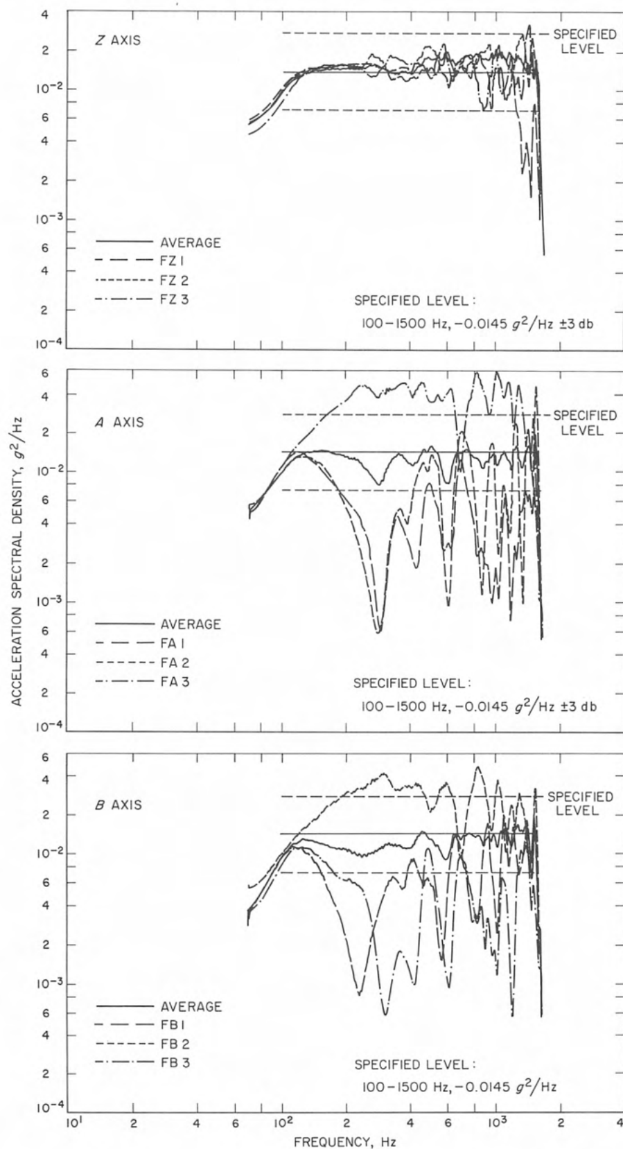
Fig. X-11. SC-7 random vibration test input level vs specification values
