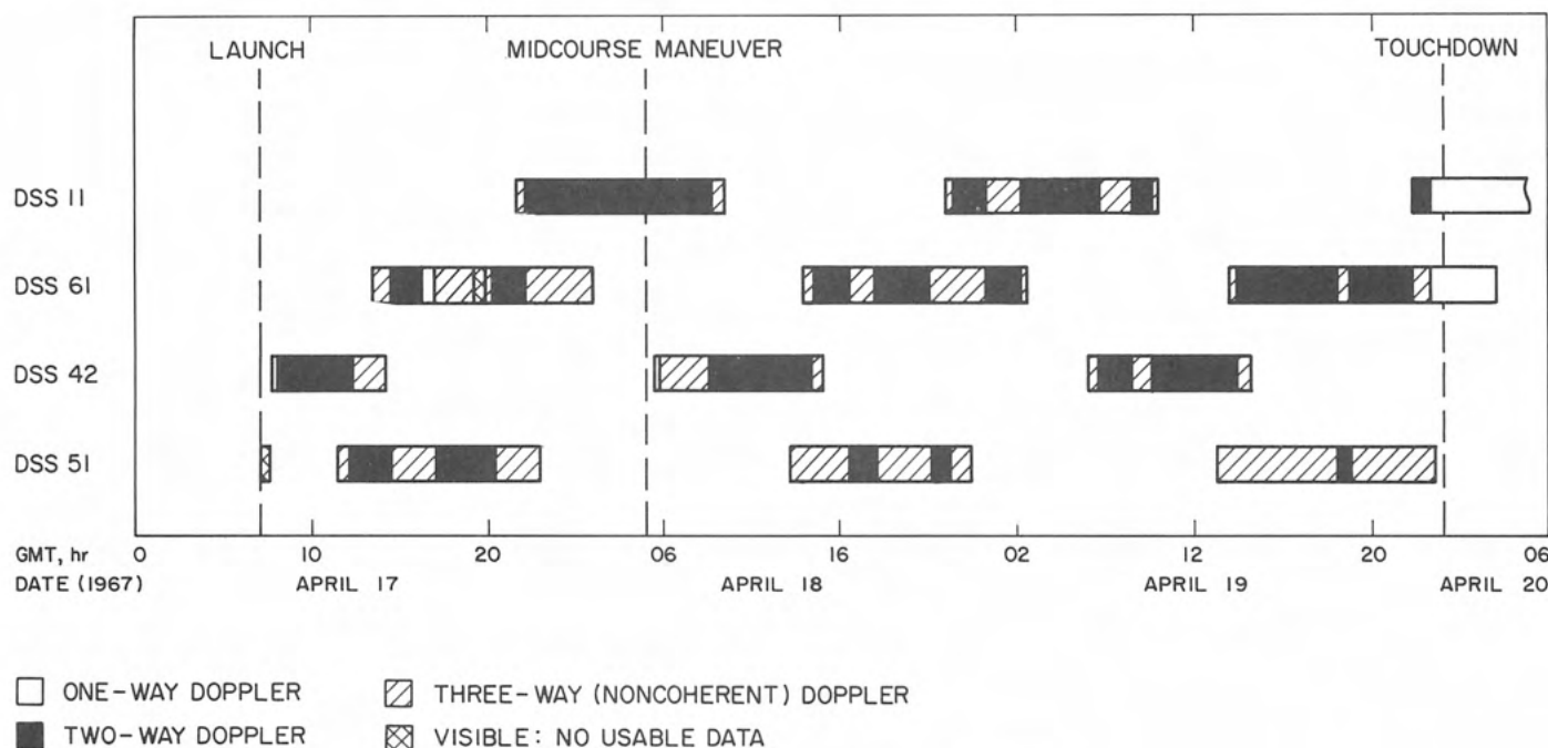
Fig. VI-18. Tracking coverage for Surveyor III
