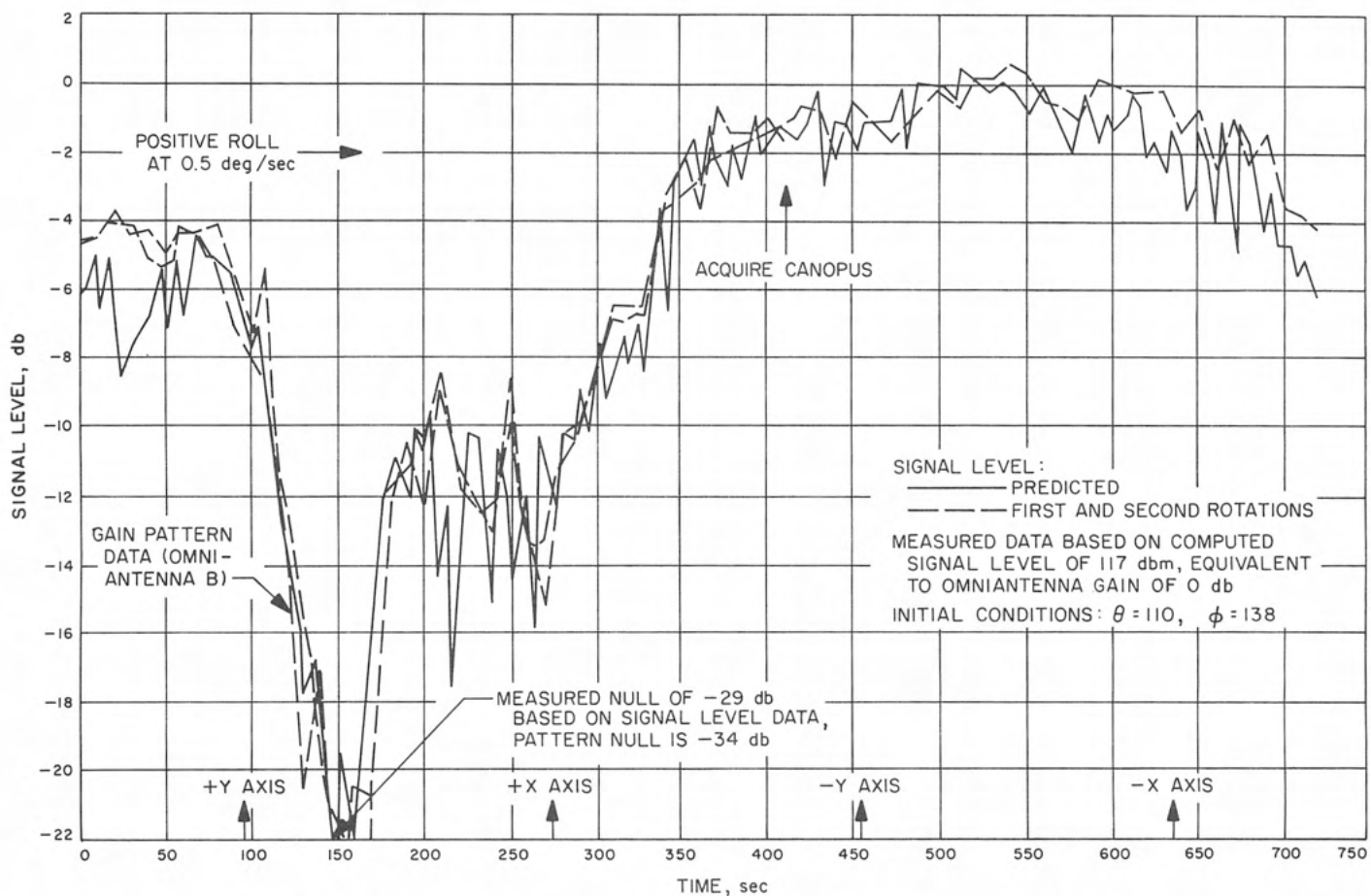
Fig. VI-43. Surveyor III signal level vs predictions during star acquisition for omniantenna B downlink
