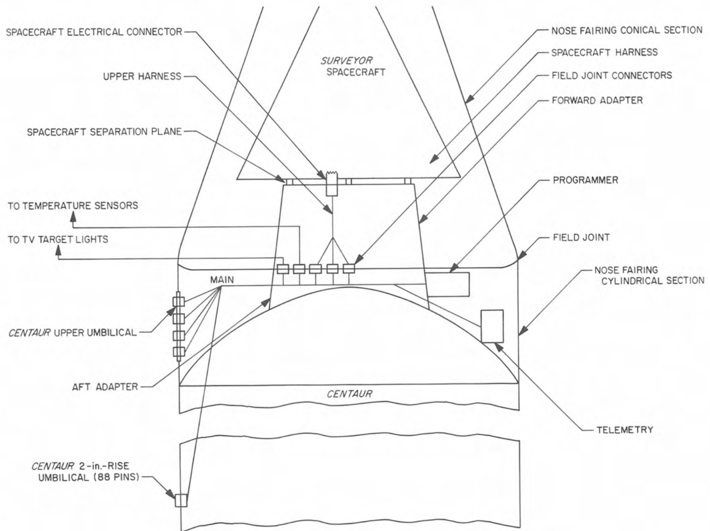
Fig. VIII-23. Centaur/Surveyor internal wiring scheme
