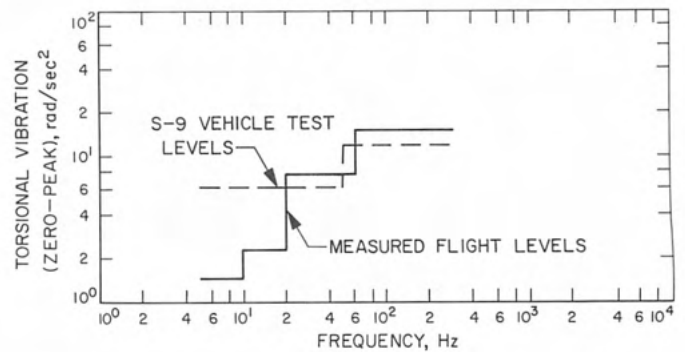
Fig. X-16. Comparison of the 95% flight equivalent torsional sinusoidal vibration environment and the specified torsional sinusoidal vibration environment for the S-9 structural test vehicle
