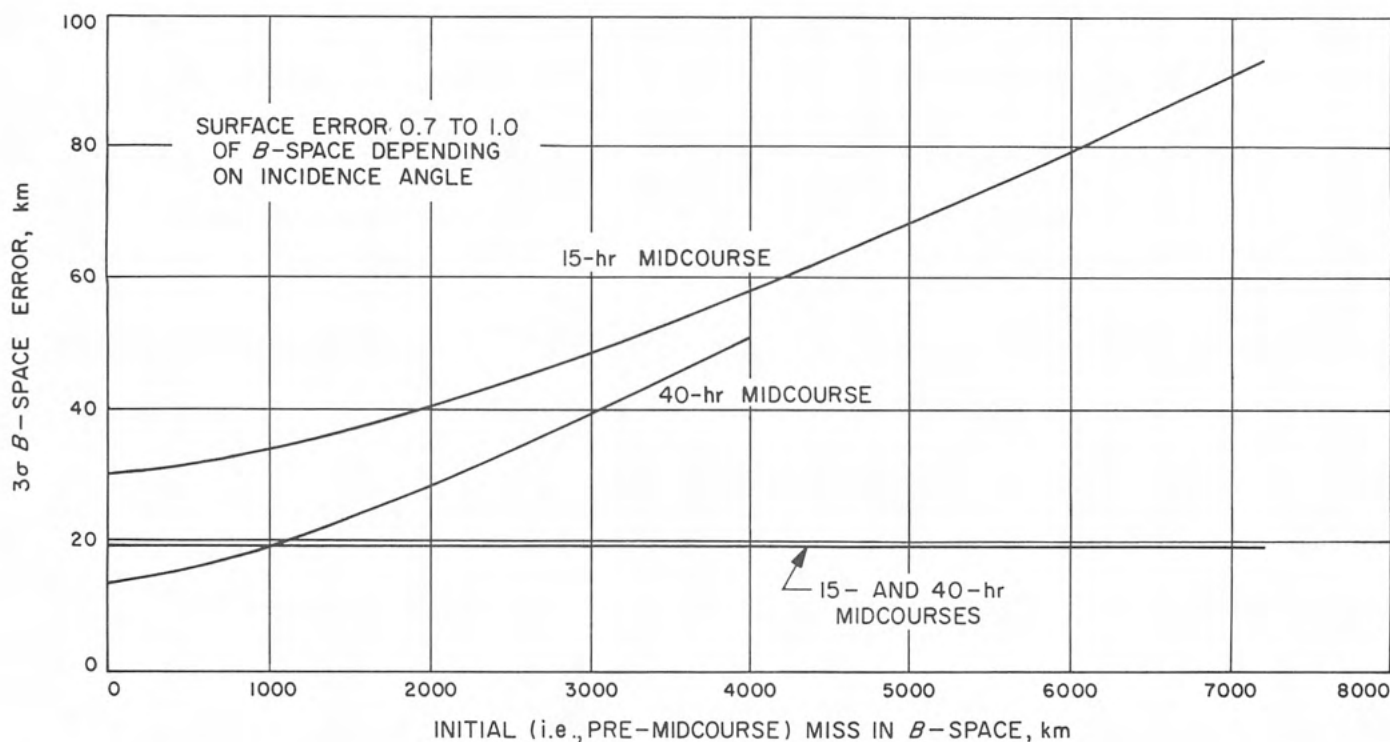
Fig. VI-25. Guidance accuracy
