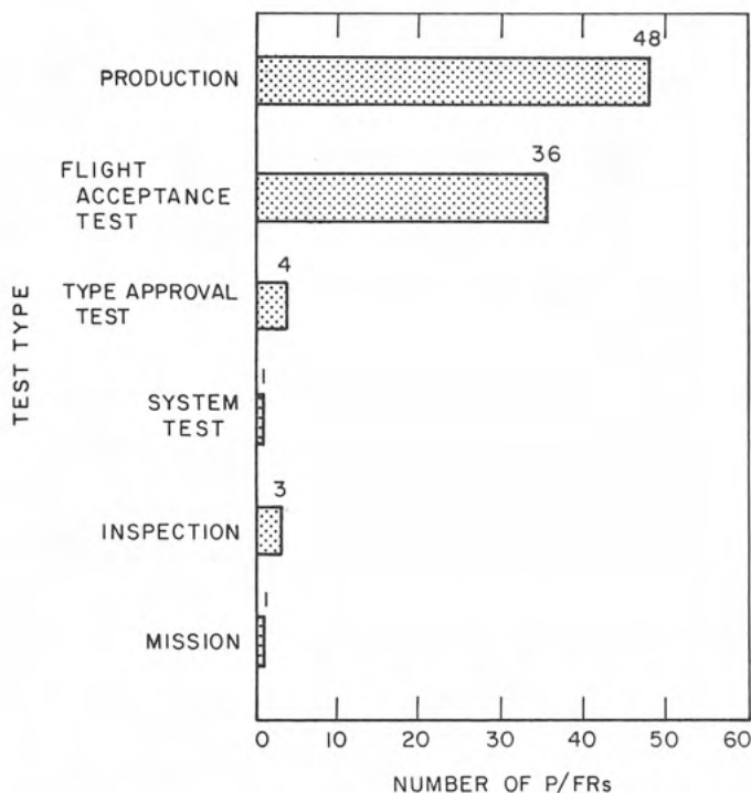
Fig. XII-17. Surveyor alpha scattering instrument problem/failure reports by test type
