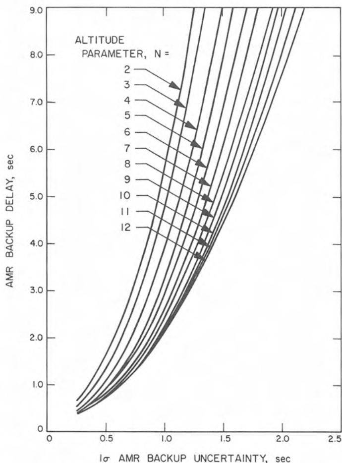
Fig. VI-26. AMR backup delay time (radar reliability: 0.999)
