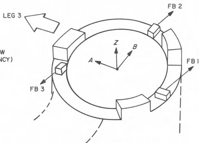
(d) CONTROL ACCELEROMETERS FOR B AXIS (LOW FREQUENCY AND SINE-RANDOM)
