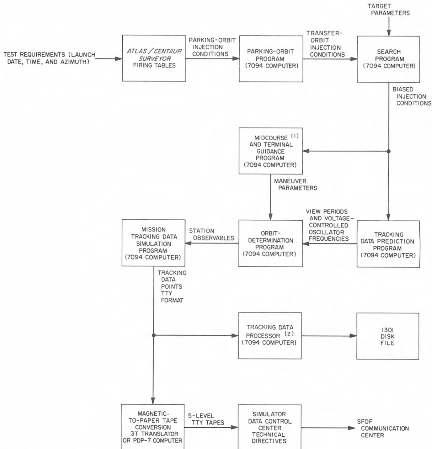
Fig. VII-13. Simulated tracking data generation sequence
