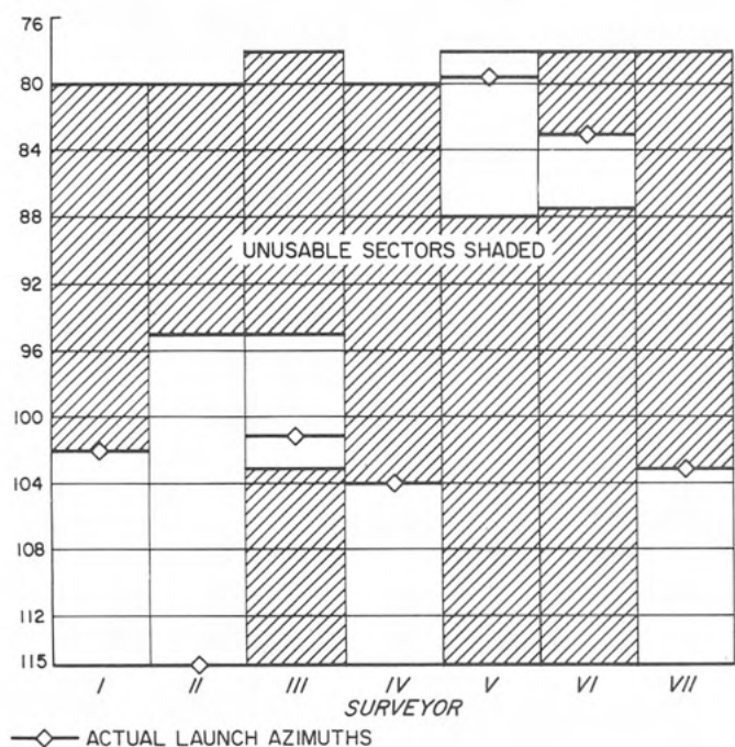
Fig. VI-17. Final launch window designs (including refinements made during countdowns) and actual launch azimuths
