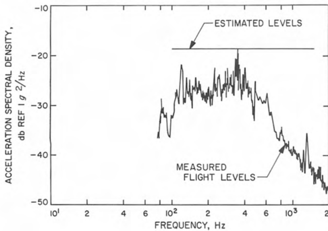
Fig. X-13. Comparison of the 95% flight random vibration environment and the estimated random vibration environment for both longitudinal and lateral axes
