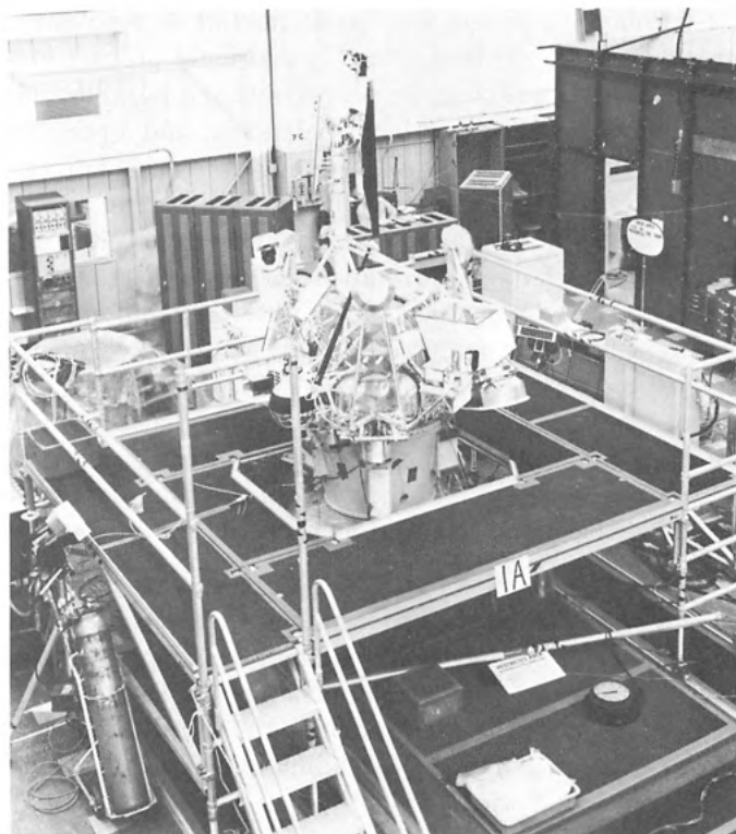
Fig. IX-6. Setup for vibration tests showing workstand
