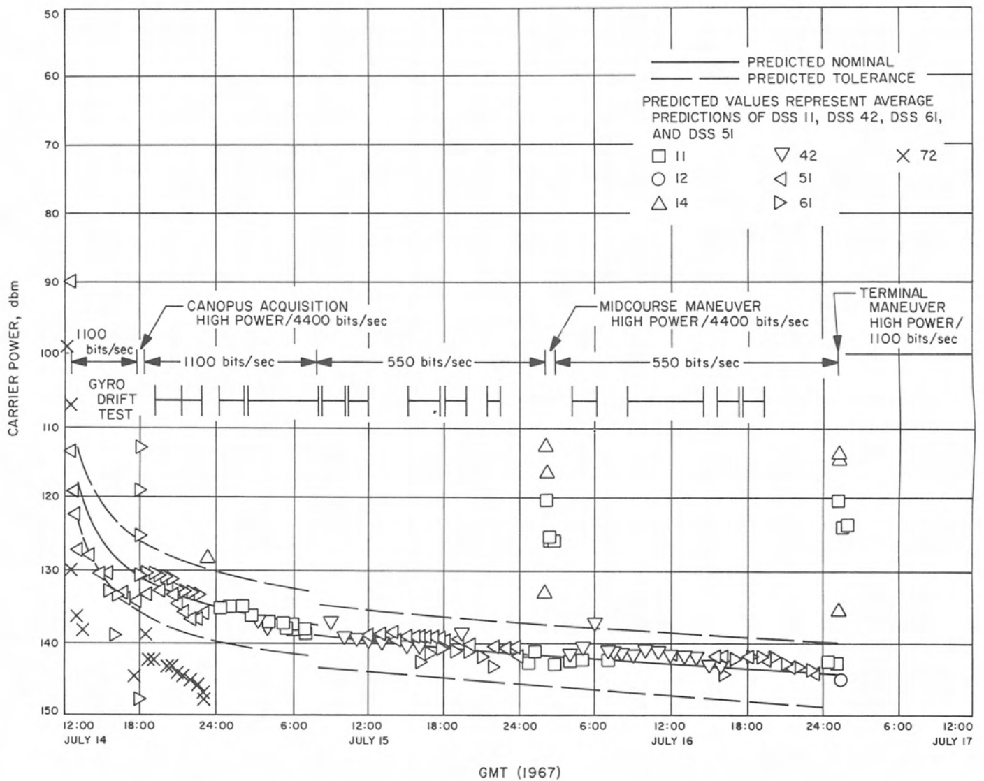
Fig. VI-37. Predicted signal levels for Surveyor IV: DSS received carrier power
