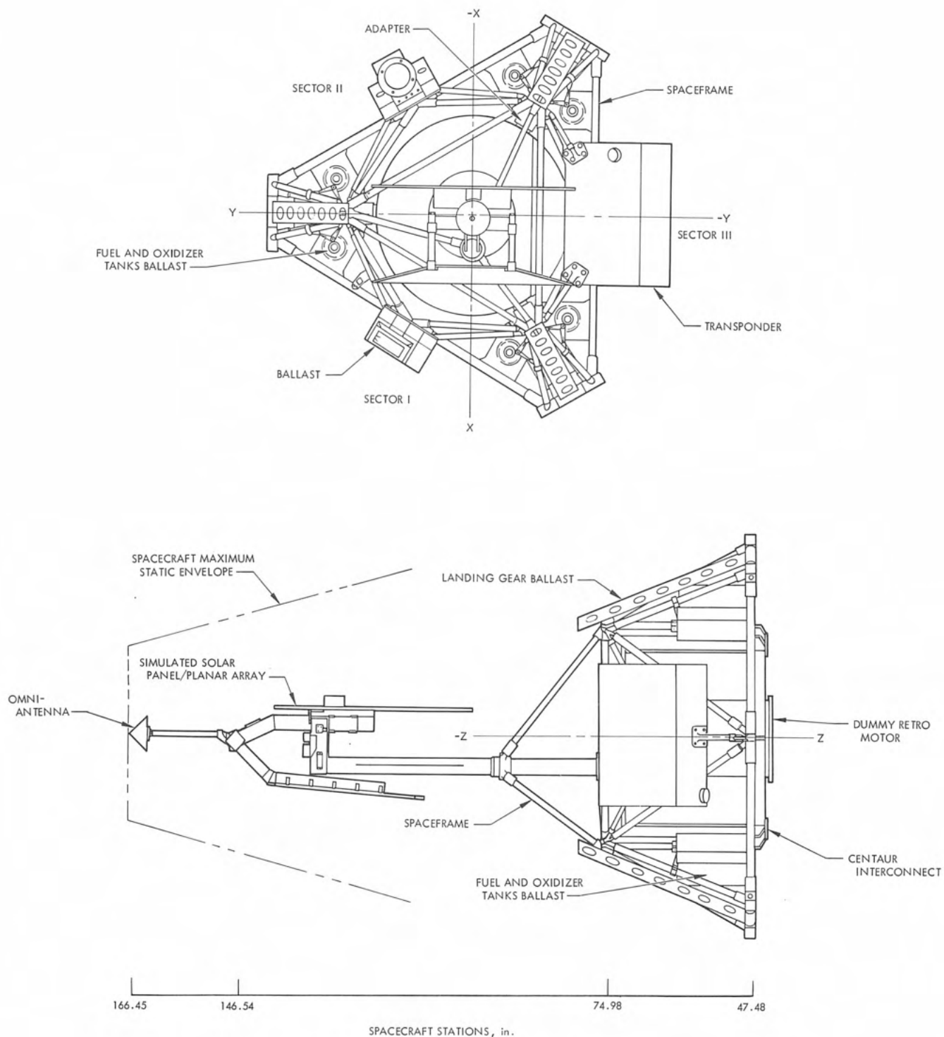
Fig. XI-26. Dynamic model top and side view
