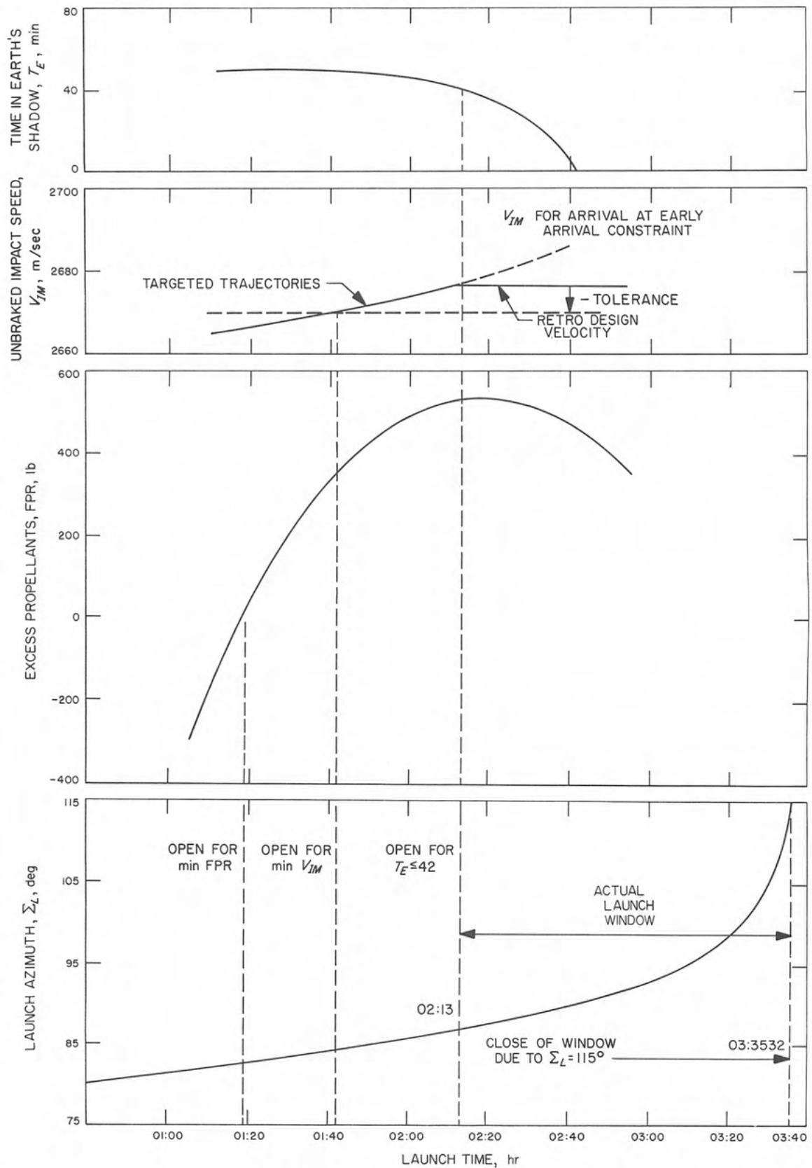
Fig. VI-35. Sample launch window refinement
