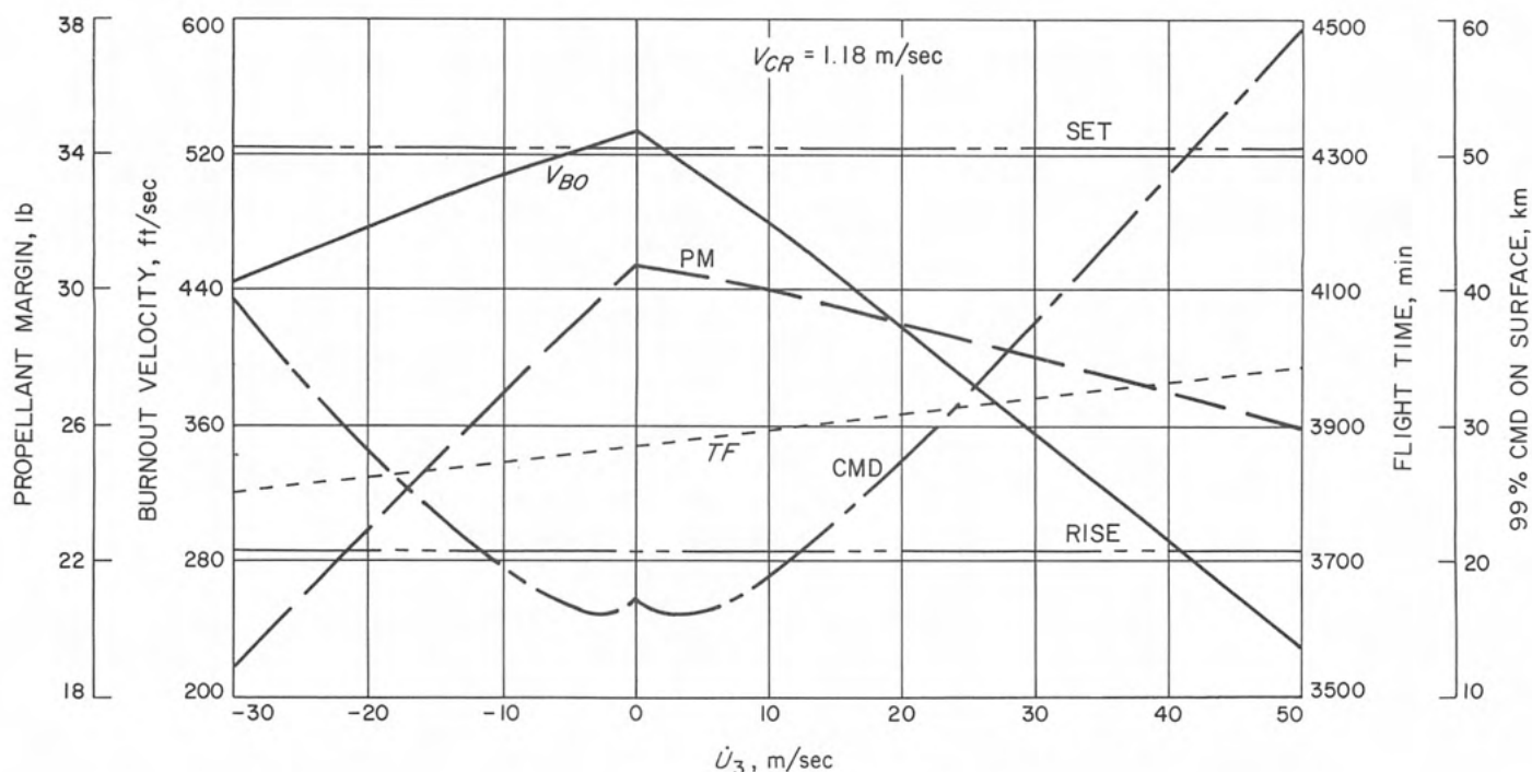
Fig. VI-21. Typical \dot{U}_3 scan
