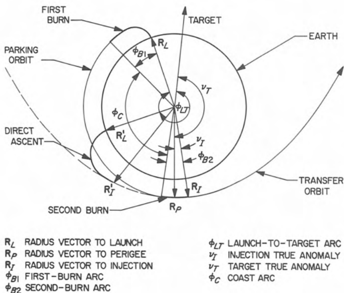
Fig. VI-10. Parking-orbit vs direct-ascent geometry
