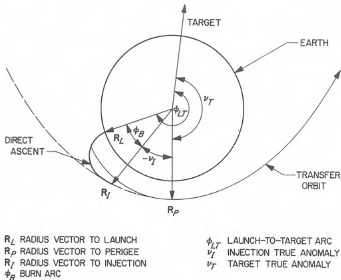
Fig. VI-5. In-plane direct-ascent geometry
