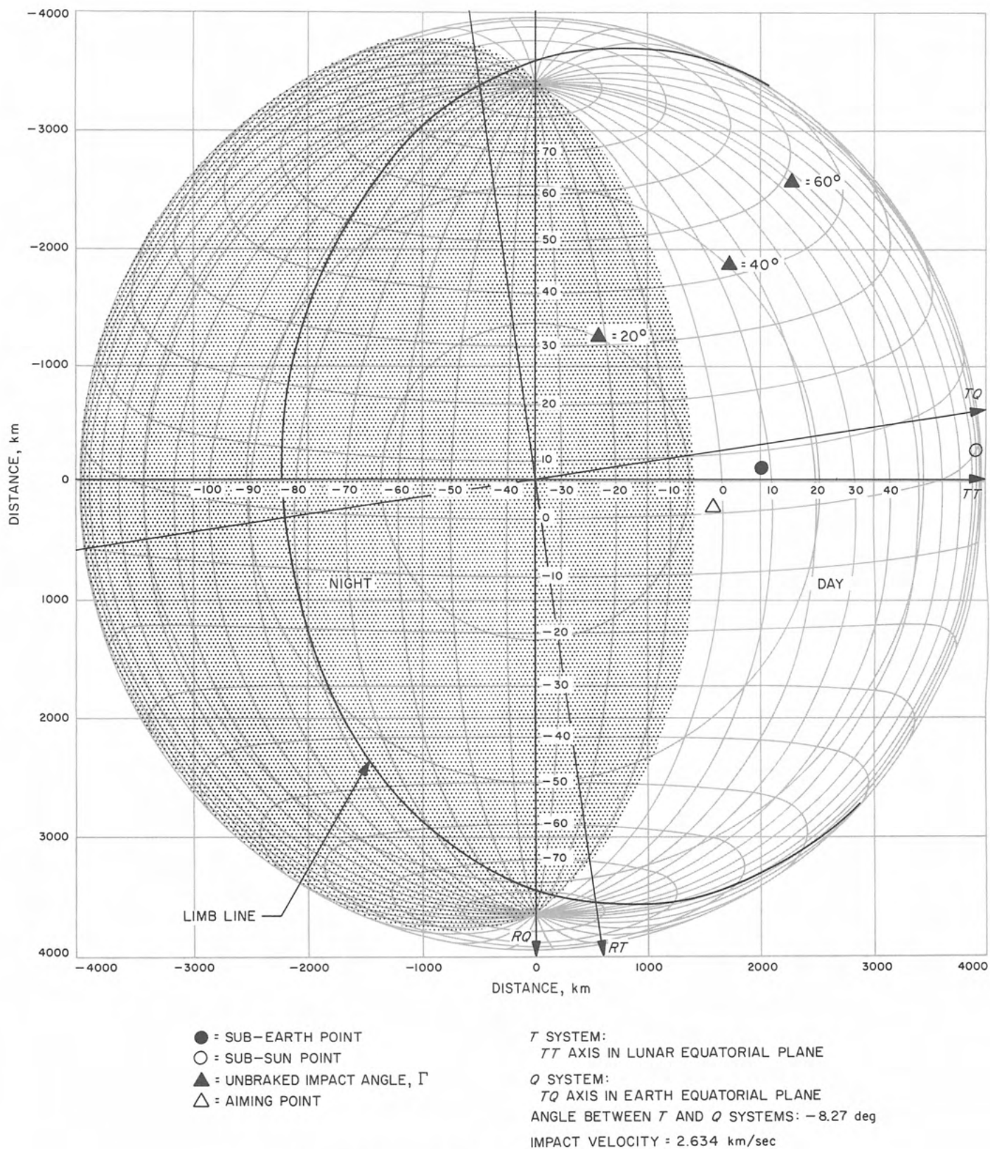
Fig. VI-20. Moon in B-space for typical trajectory
