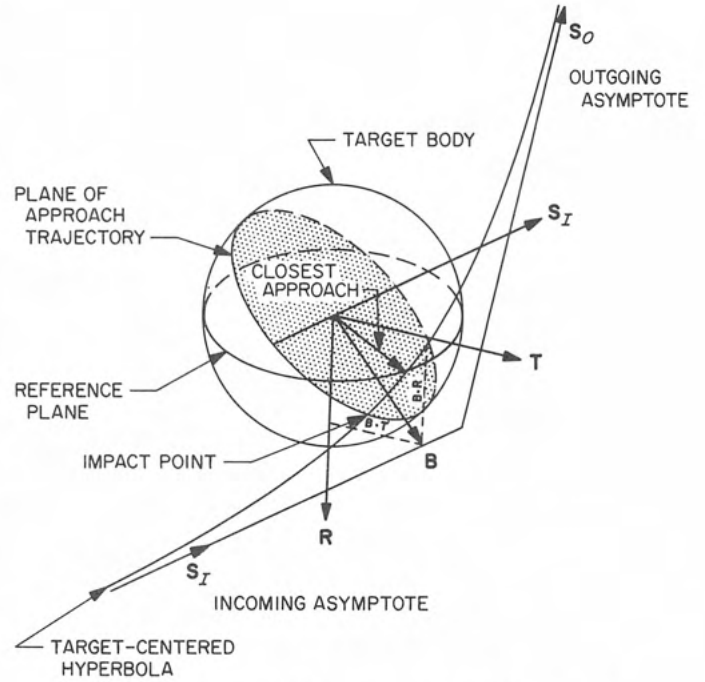
Fig. VI-19. Definition of \mathbf{B} \cdot \mathbf{T} , \mathbf{B} \cdot \mathbf{R} system
