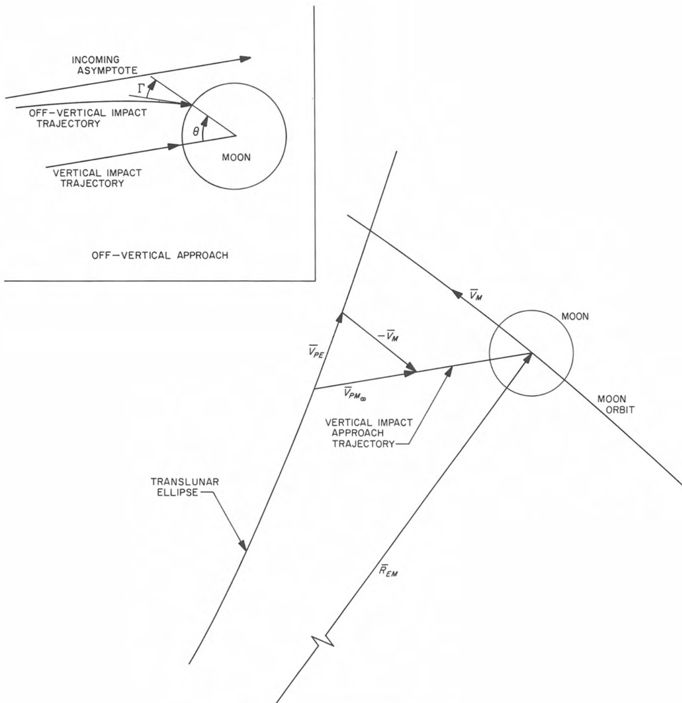
Fig. VI-4. Lunar encounter geometry
