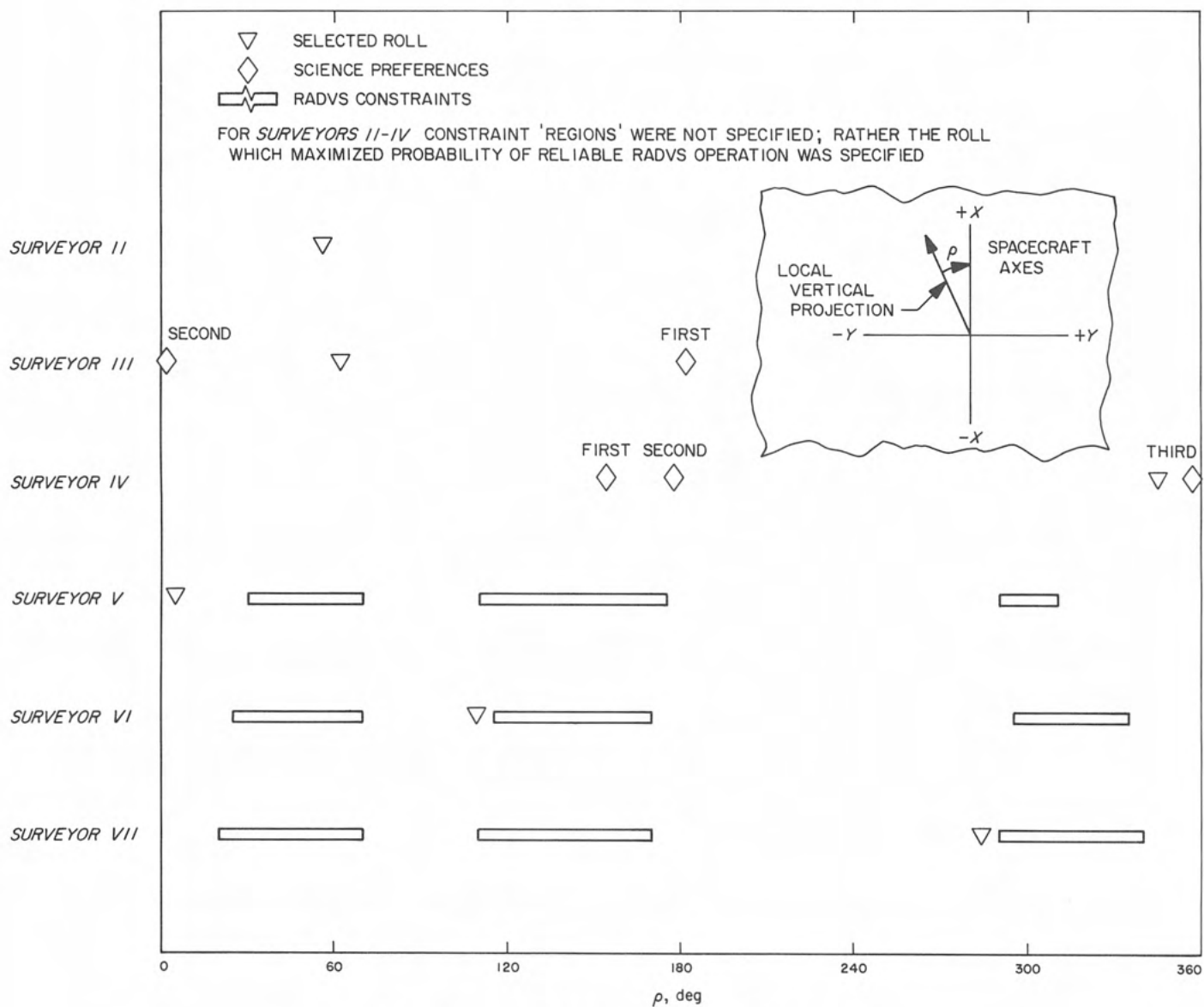
Fig. VI-27. Roll attitude constraints and selections
