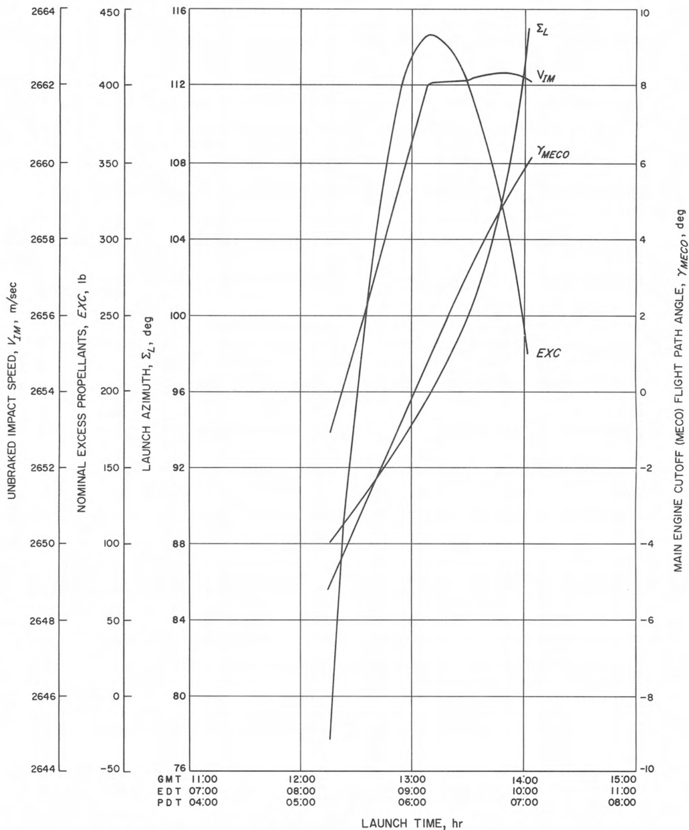
Fig. VI-30. Typical graph of unbraked impact speed, nominal excess propellants, launch azimuth, and MECO flight path angle vs launch time
