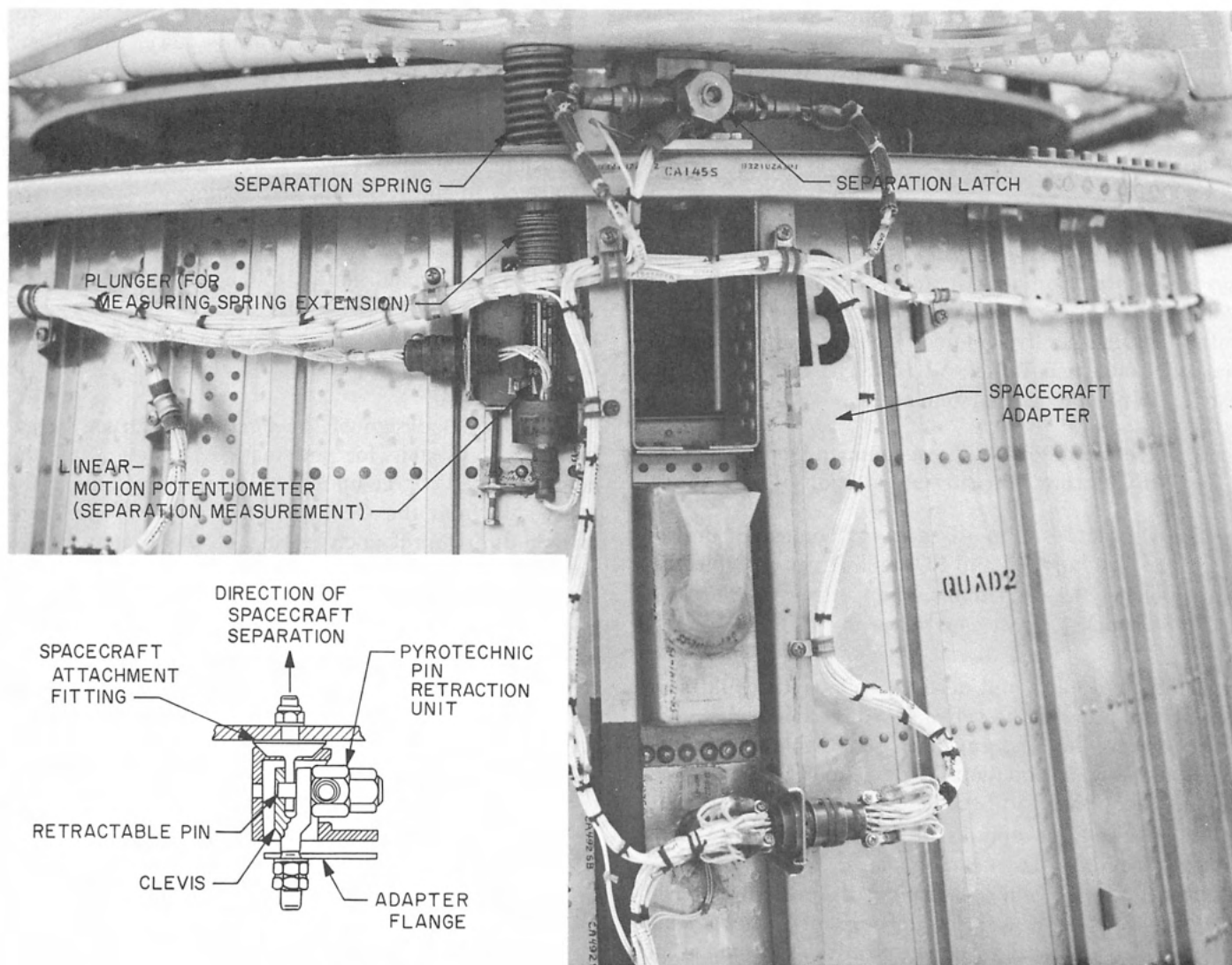
Fig. VIII-12. Payload separation mechanism and instrumentation
