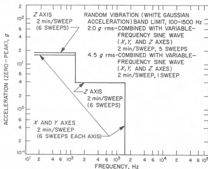
Fig. X-4. Typical TA vibration test requirements for control items
