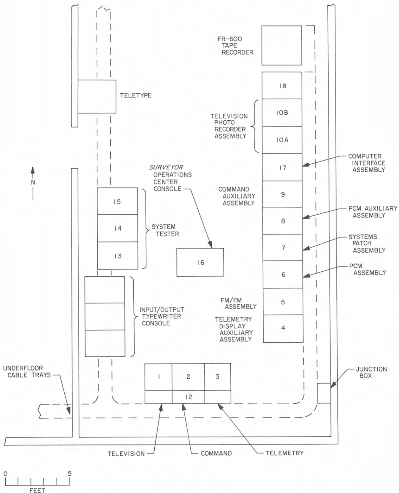
Fig. VII-6. Floor plan of CDC 1 at DSS 11
