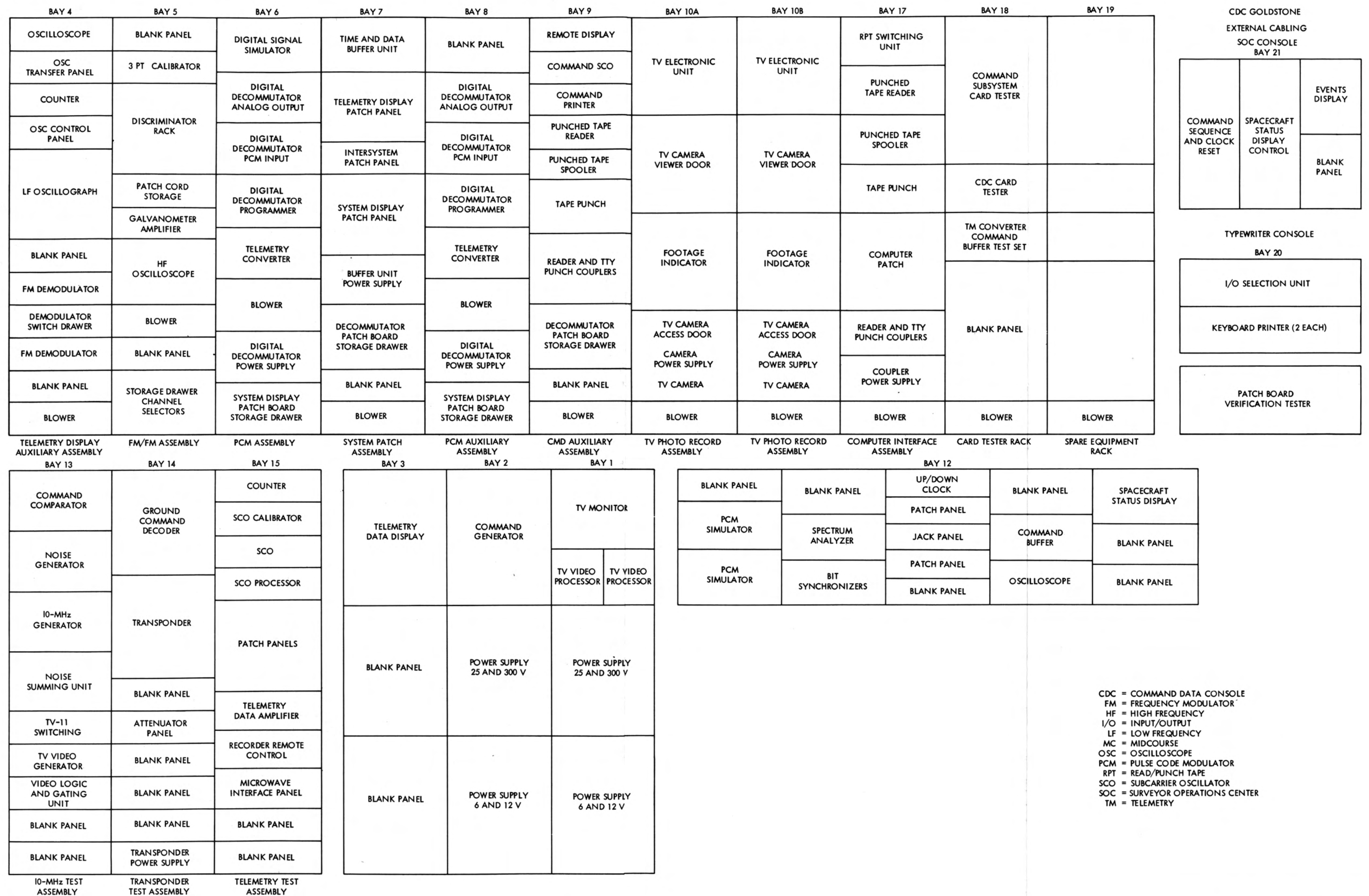
Fig. VII-5. Equipment layout in CDC racks
