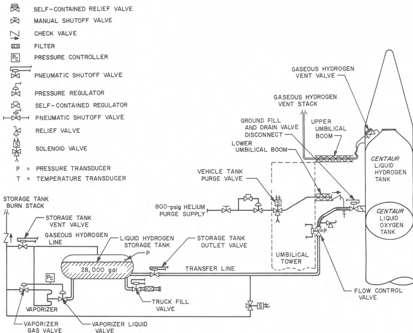
Fig. VIII-26. Liquid hydrogen transfer system, Launch Complex 36
