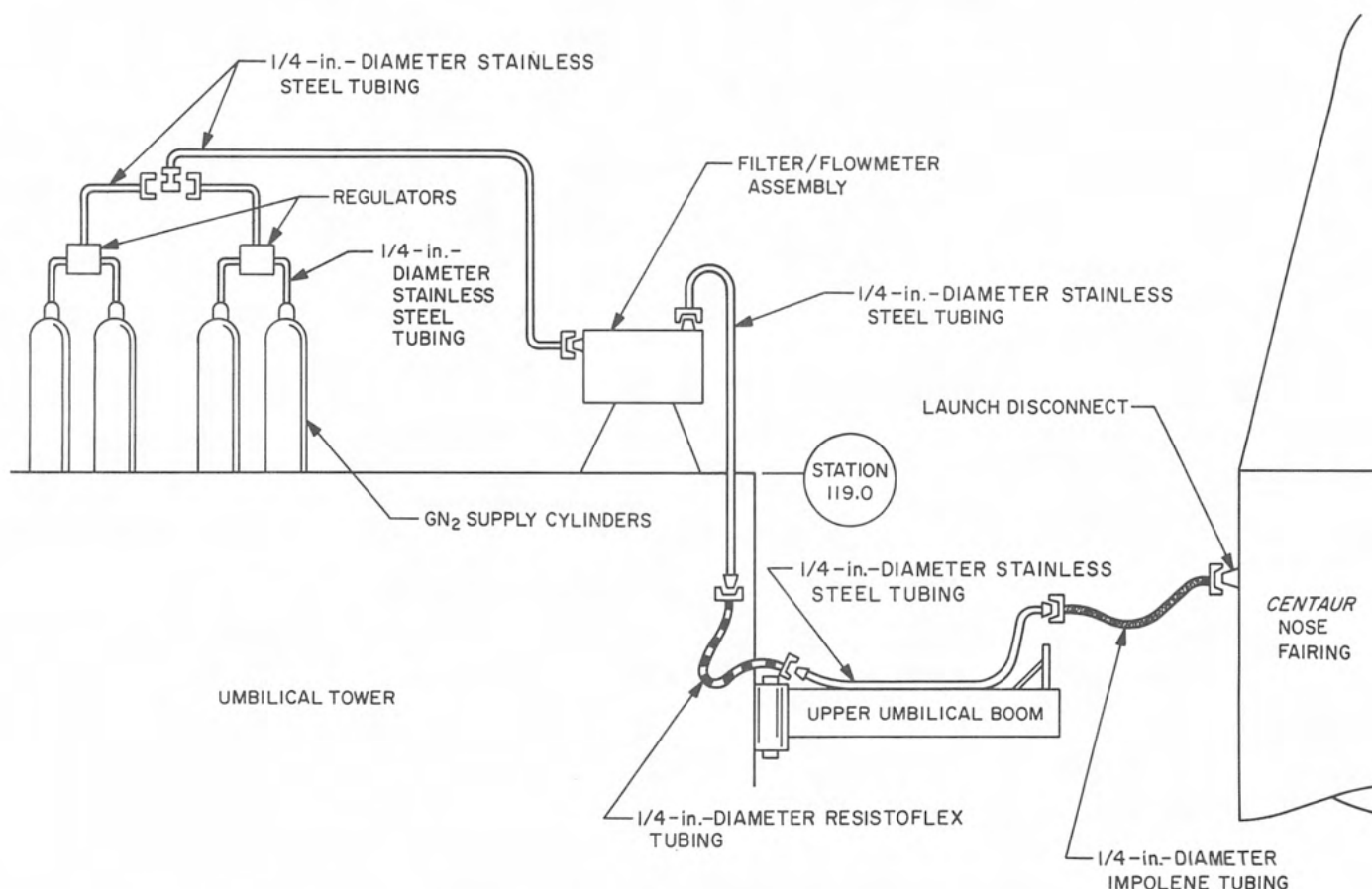
Fig. VIII-19. Alpha scattering instrument gaseous nitrogen purging system
