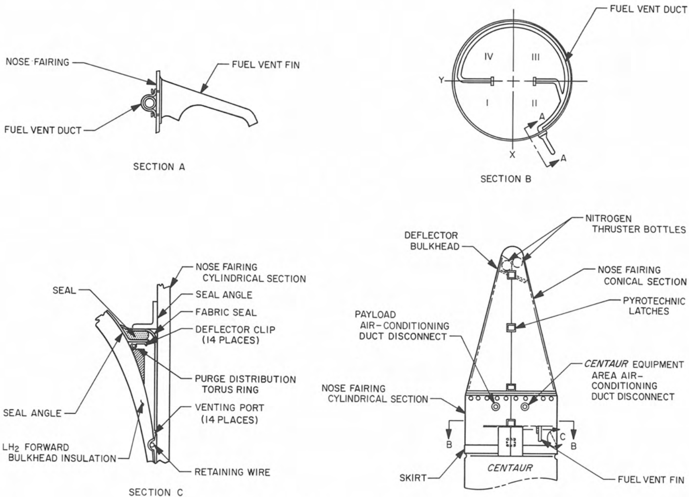
Fig. VIII-8. Nose fairing, general arrangement
