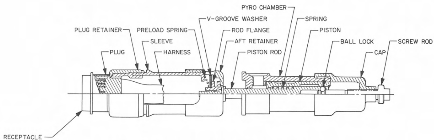
Fig. VIII-13. Electrical connector separation mechanism
