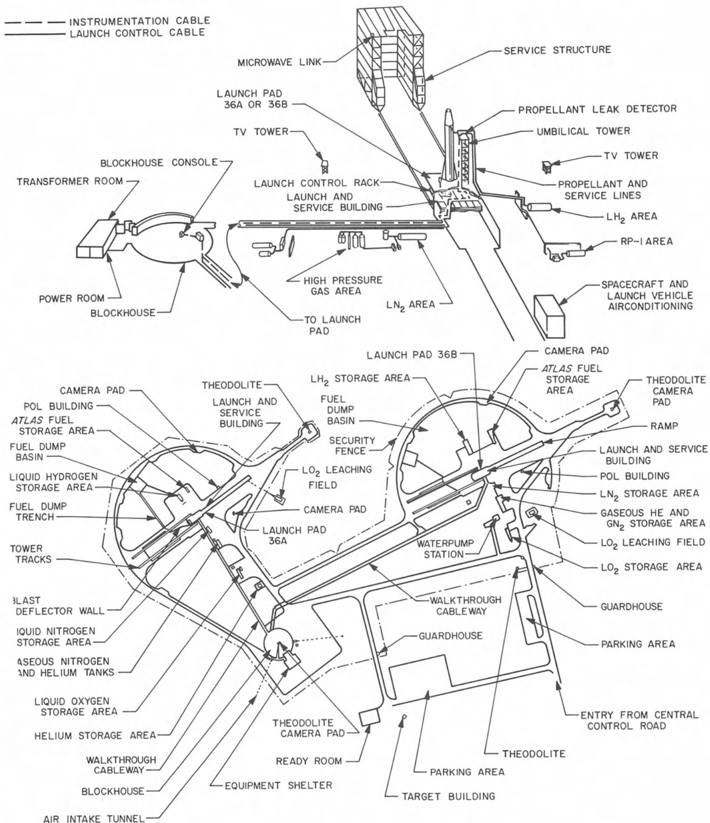
Fig. VIII-22. Launch Complex 36 configuration
