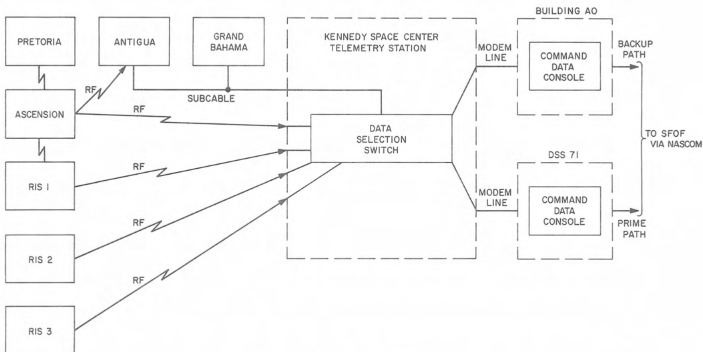
Fig. VII-21. Surveyor real-time spacecraft telemetry data transmission system
