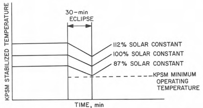
Fig. X-2. Determination of the 87% solar constant test level
