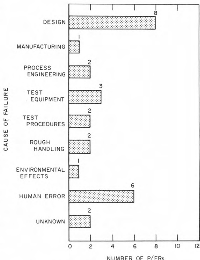
Fig. XII-12. Surveyor GFE solar-panel P/FRs listed by failure cause
