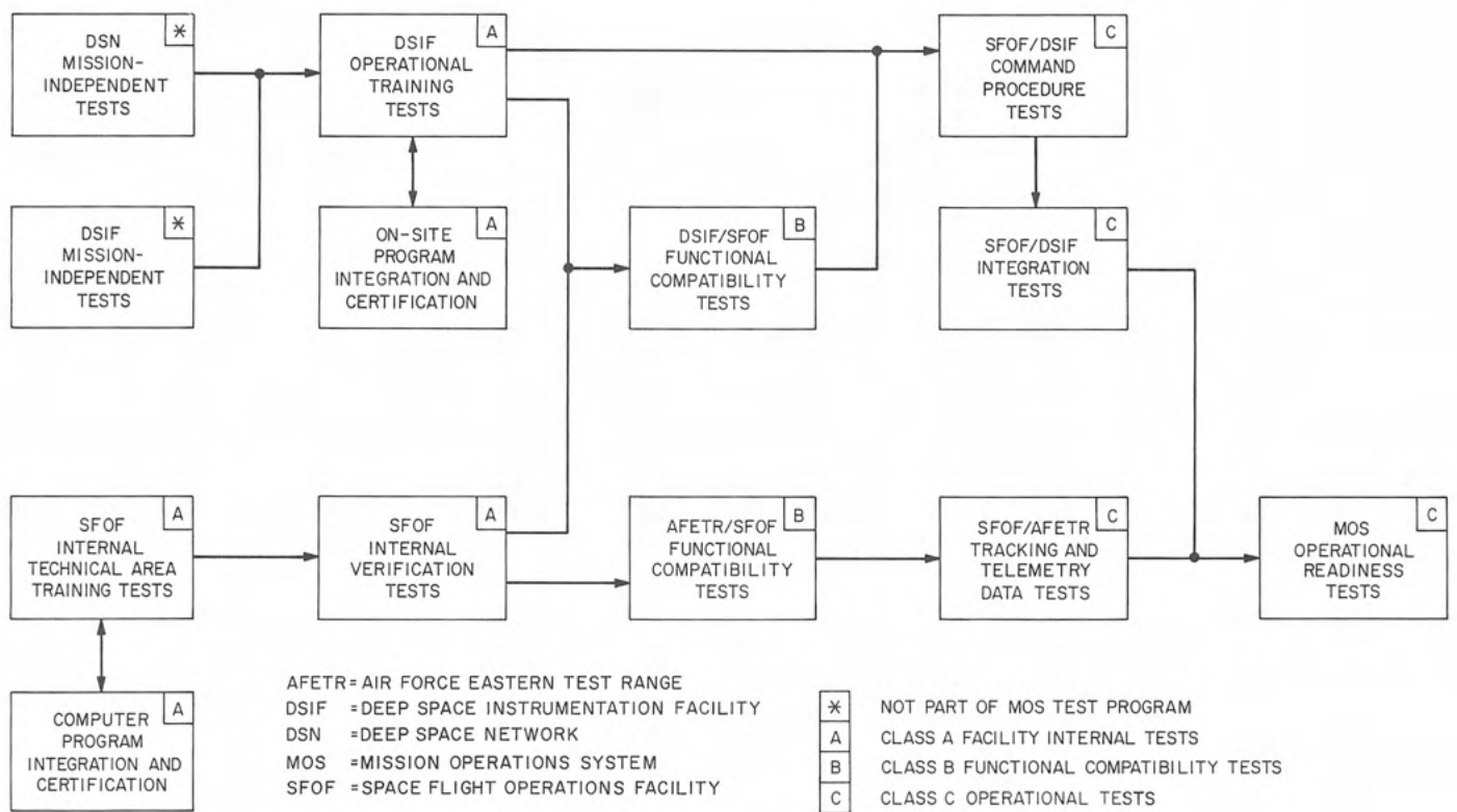
Fig. VII-16. Relationship of MOS tests
