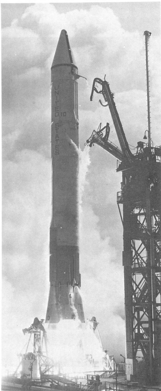
Fig. I-2. Atlas/Centaur (AC-10) launching Surveyor I
