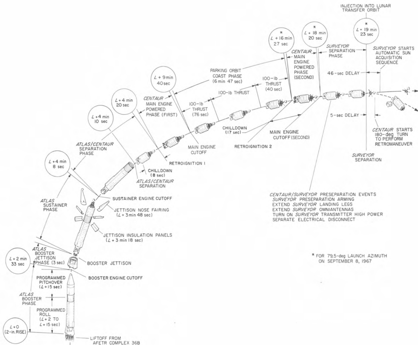
Fig. VIII-32. Surveyor V postlaunch events (parking orbit)
