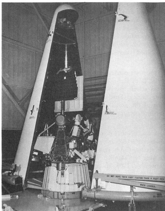
Fig. VIII-16. Spacecraft encapsulation
