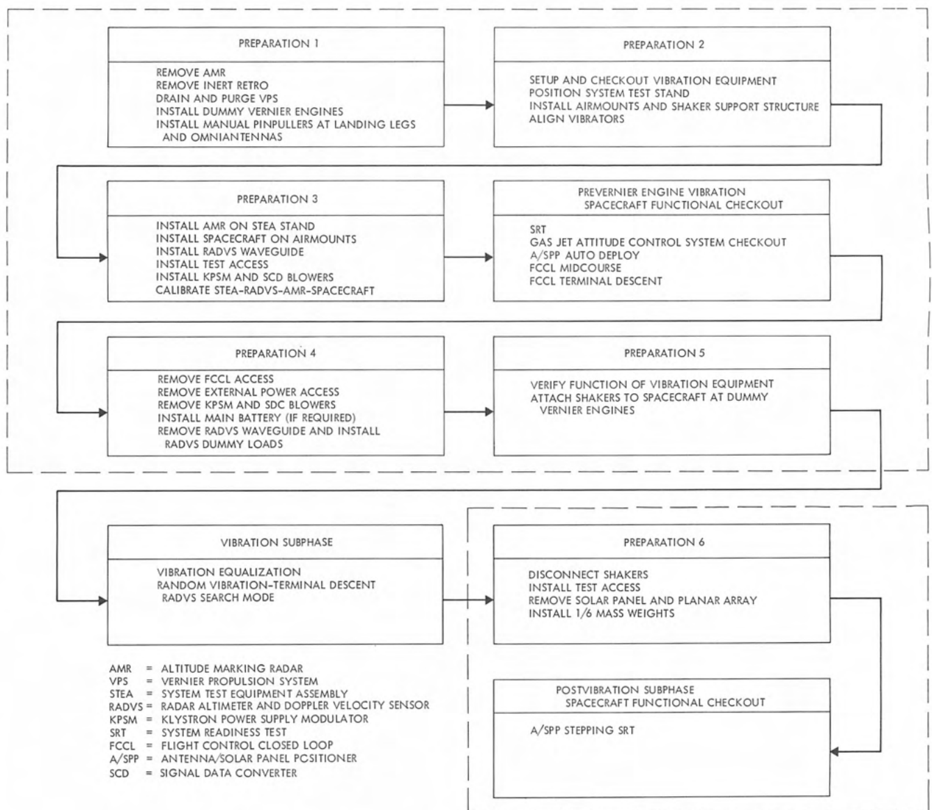
Fig. XI-16. Vernier engine vibration phase flow diagram
