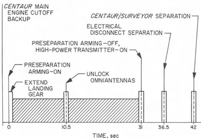
Fig. VIII-15. Spacecraft/ Centaur separation sequence commands
