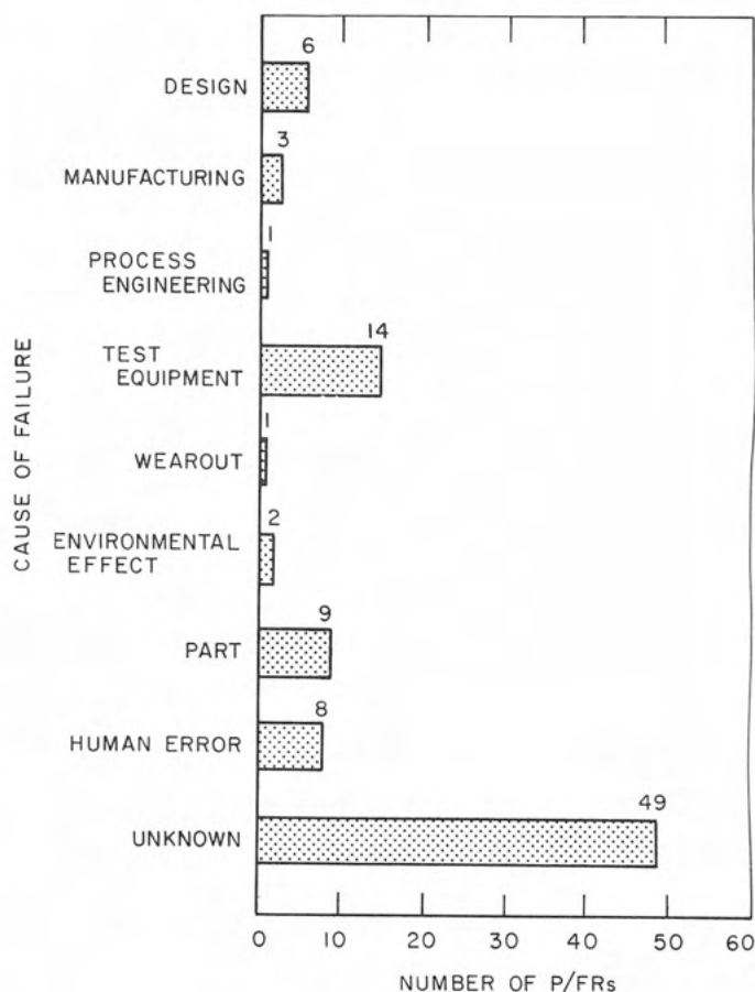
Fig. XII-16. Surveyor alpha scattering instrument problem/failure reports by failure cause
