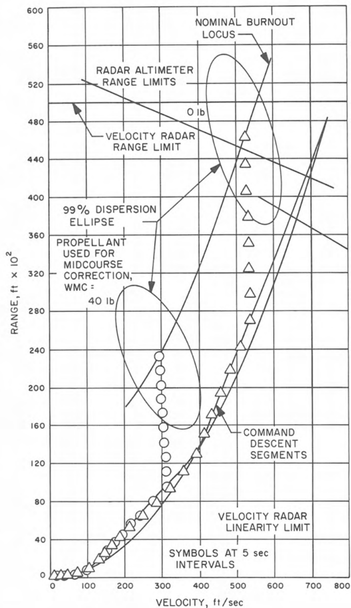
Fig. VI-23. Vernier descent phase (unbraked impact angle: 24^\circ )
