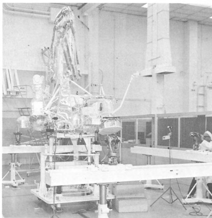
Fig. XI-18. Optical alignment dock
