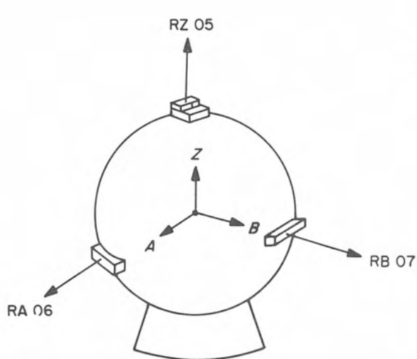
(a) RETRO MOTOR ACCELEROMETER LOCATIONS
