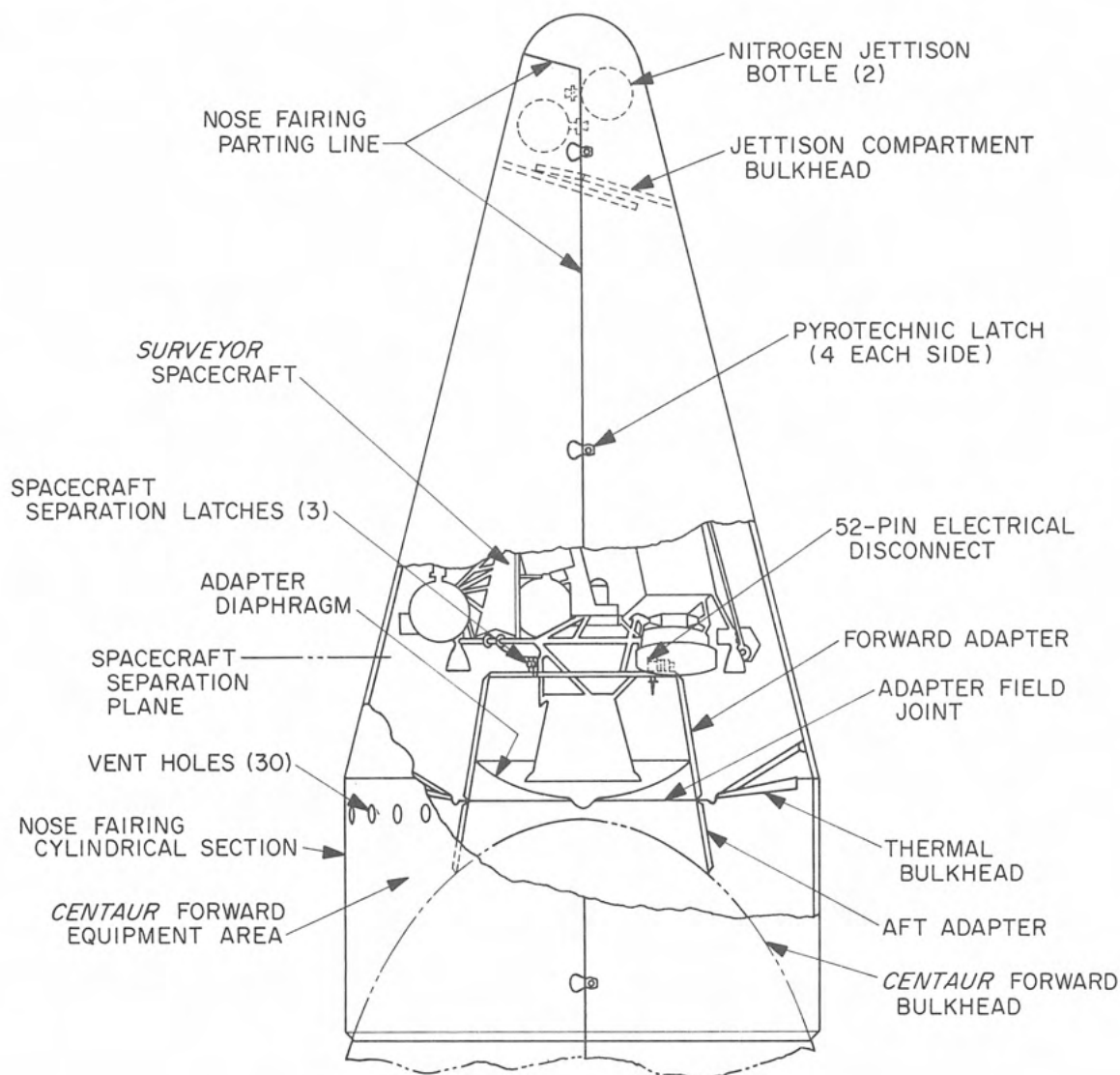
Fig. VIII-3. Surveyor/Centaur interface configuration
