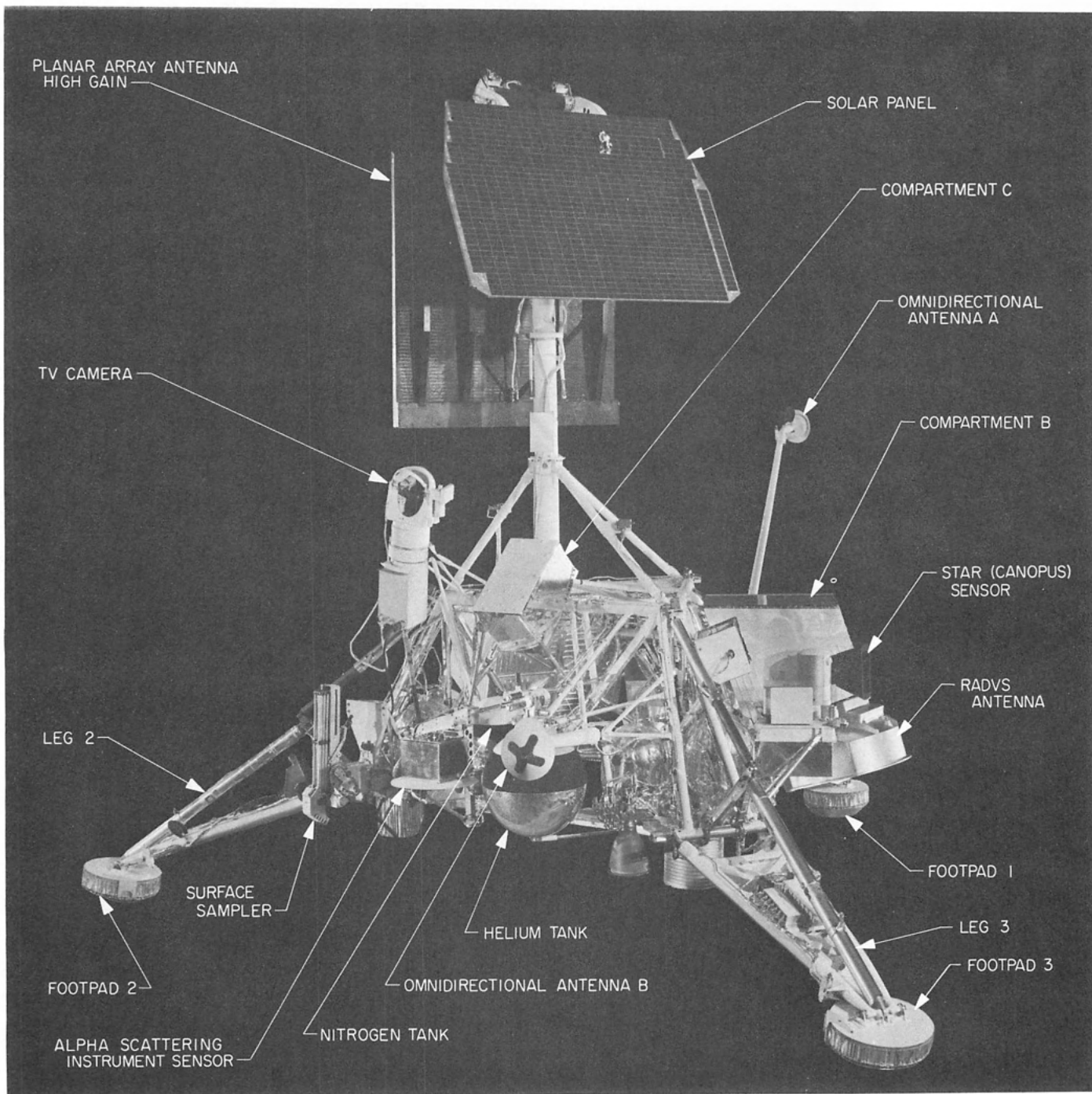
Fig. I-3. Surveyor VII spacecraft model
