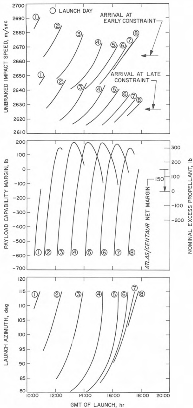
Fig. VI-14. Design chart for typical direct-ascent launch period
