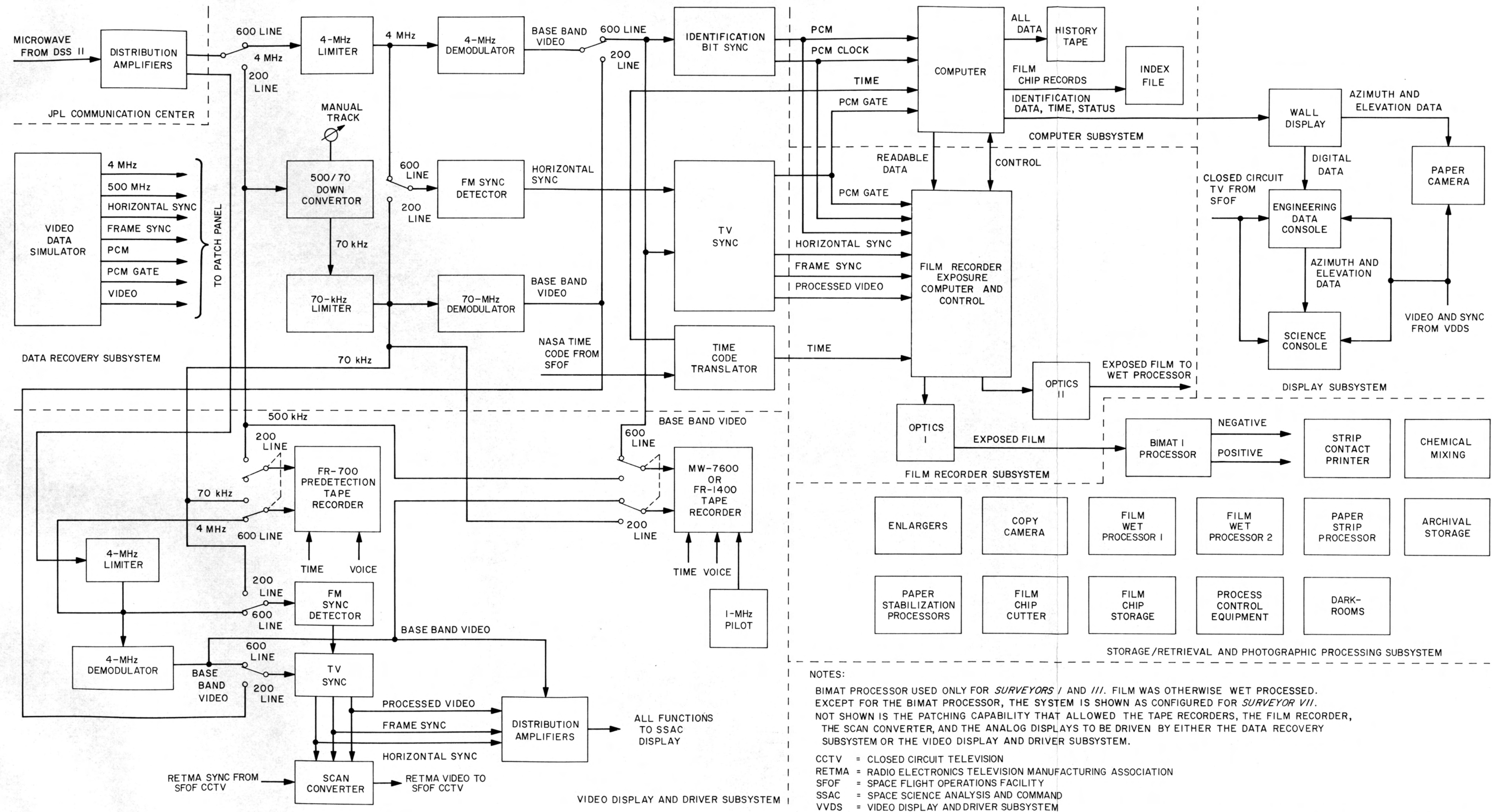
Fig. VII-10. Functional block diagram of TV-1 real-time recording mode, Surveyor Project
