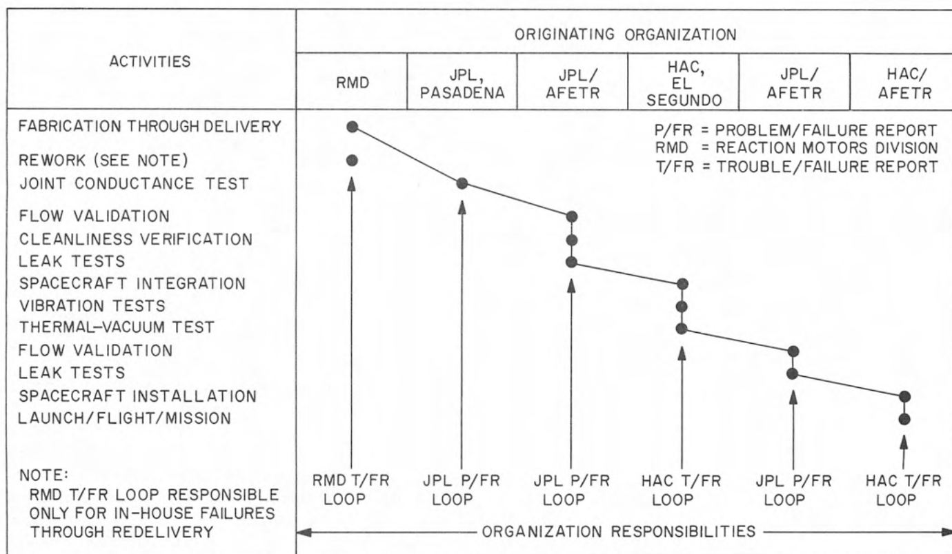
Fig. XII-19. Organizational failure reporting responsibilities as a function of post-acceptance vernier engine hardware flow
