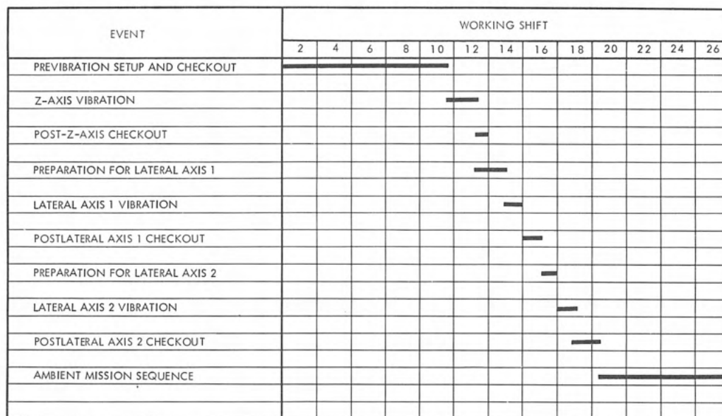
Fig. XI-15. Vibration nominal test schedule
