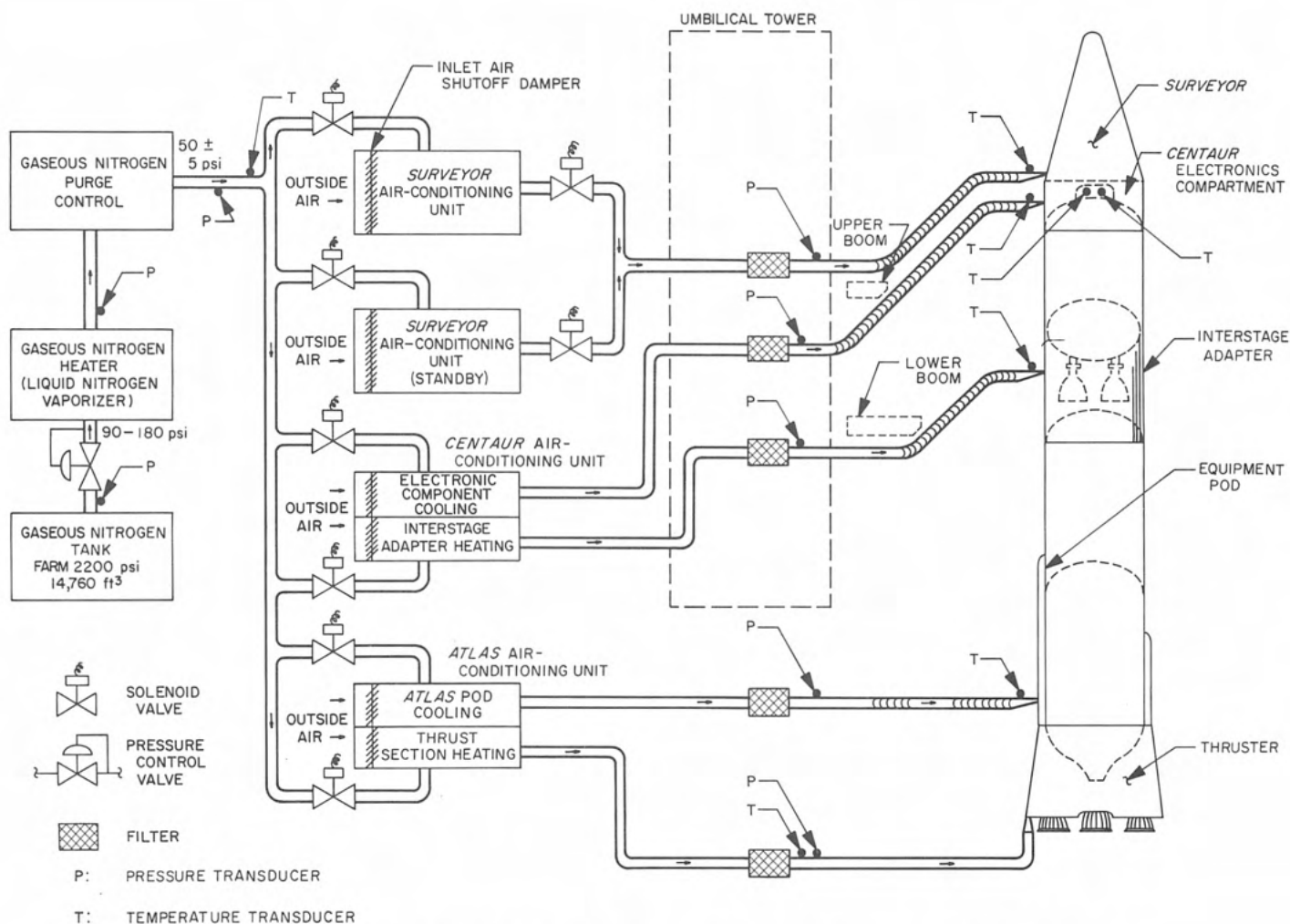
Fig. VIII-25. Atlas/Centaur/Surveyor environmental control system, Launch Complex 36
