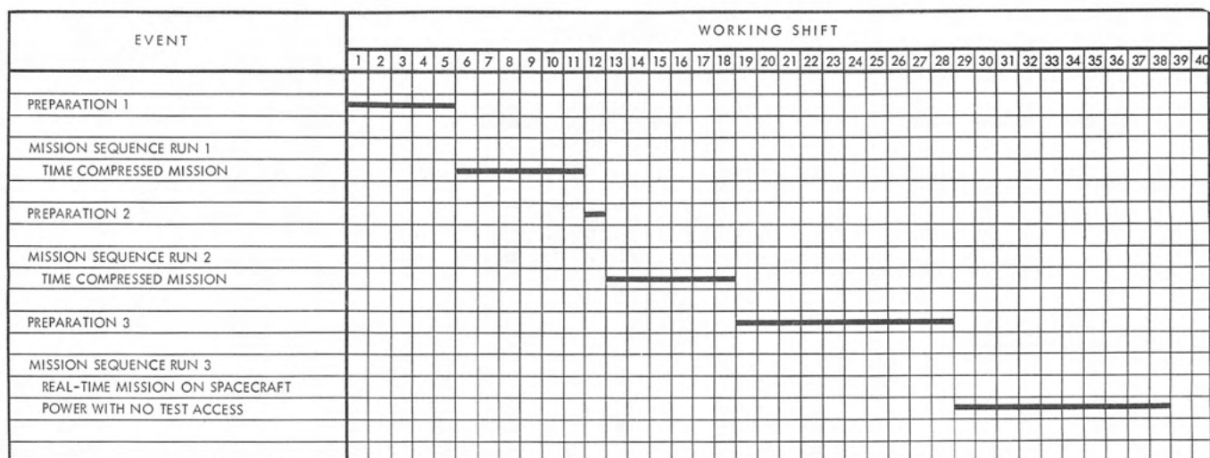
Fig. XI-9. Mission sequence/electromagnetic interference nominal test schedule
