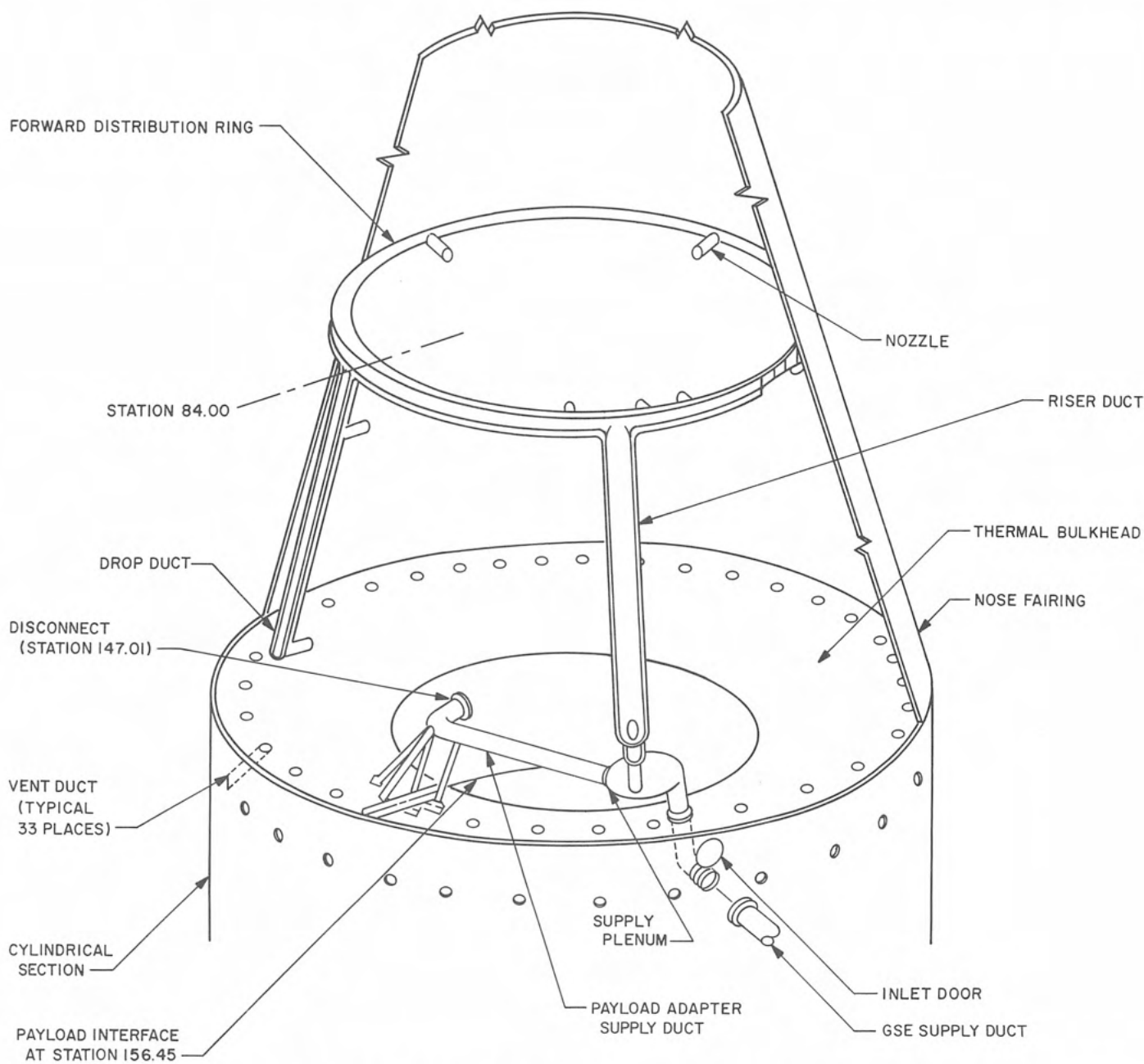
Fig. VIII-10. Spacecraft air-conditioning distribution system
