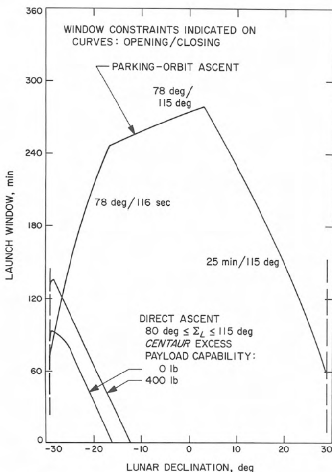
Fig. VI-11. Launch window vs lunar declination
