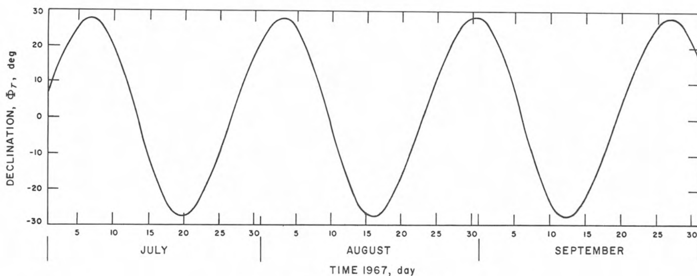
Fig. VI-12. Lunar declination vs time
