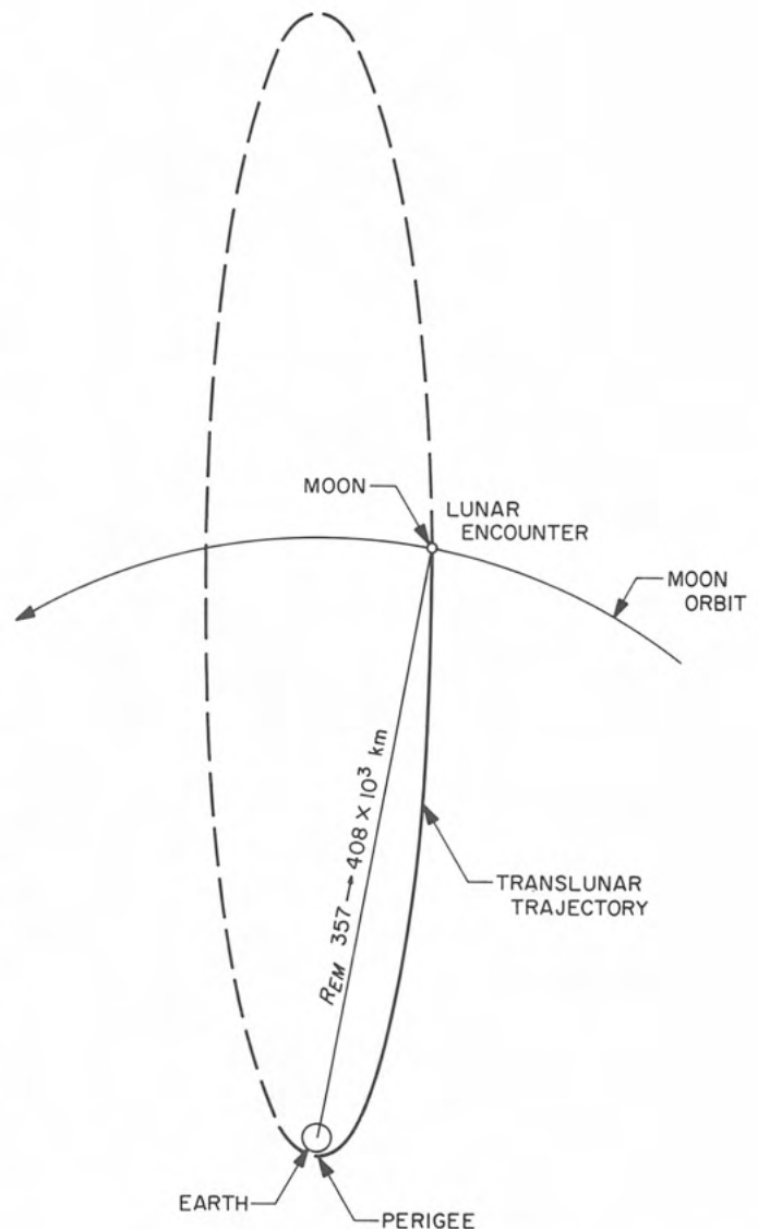
Fig. VI-2. In-plane translunar geometry (approximately to scale)
