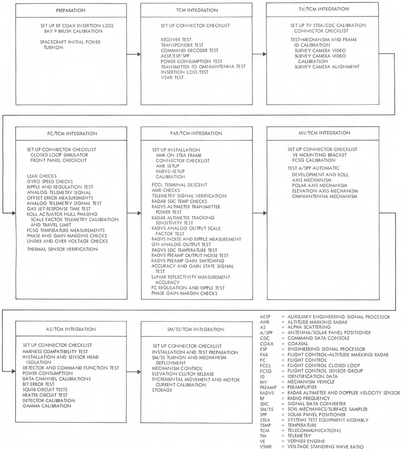
Fig. XI-6. Initial system checkout test flow diagram
