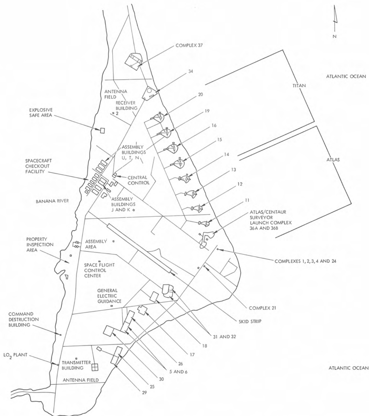
Fig. XI-22. Air Force Eastern Test Range facilities layout
