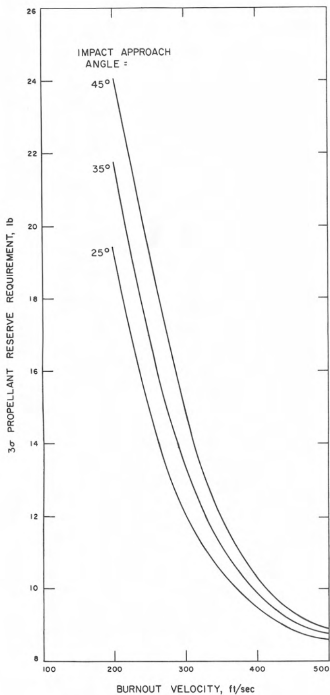
Fig. VI-22. Vernier propellant reserve
