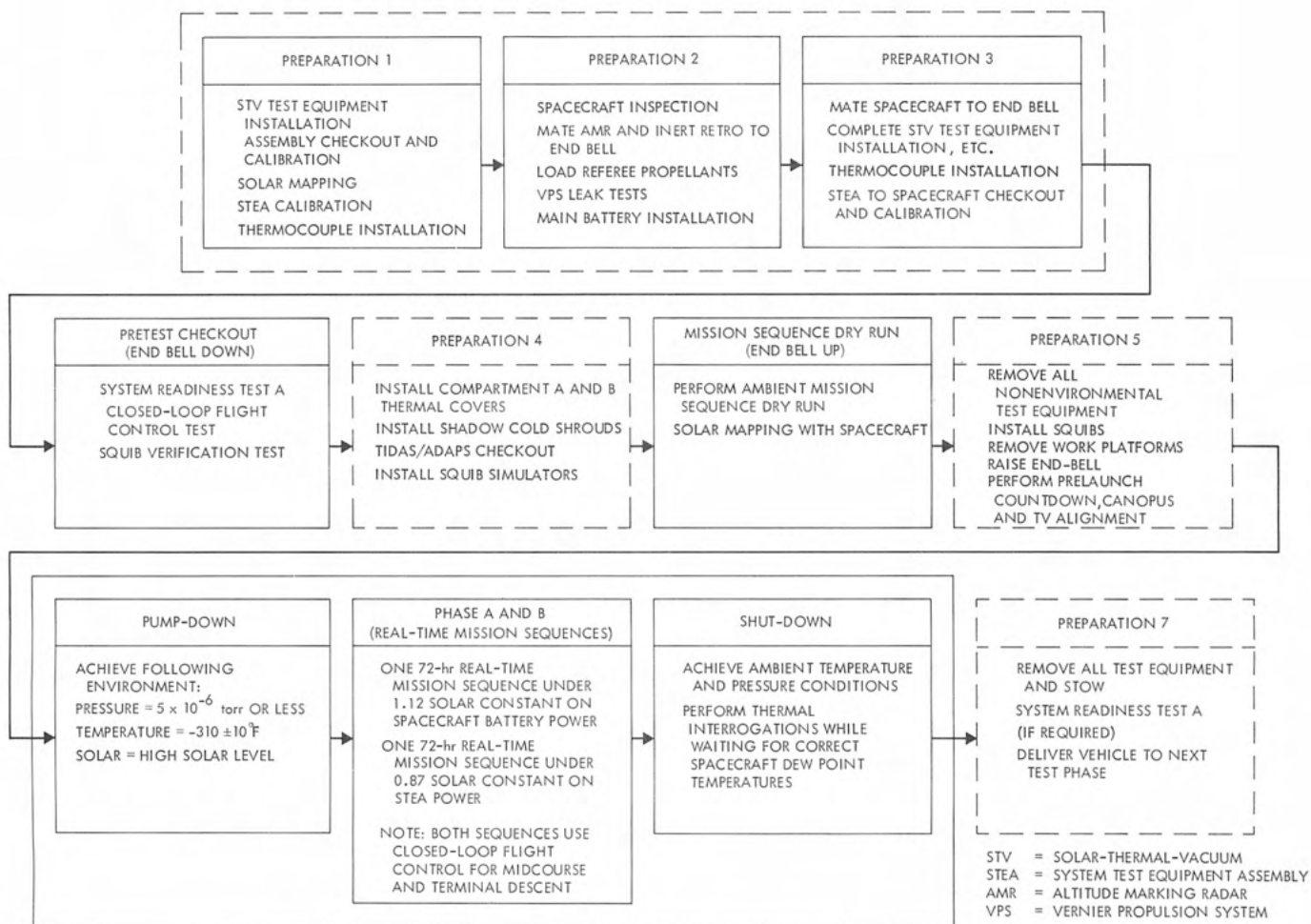
Fig. XI-10. Solar-thermal-vacuum test phase flow diagram
