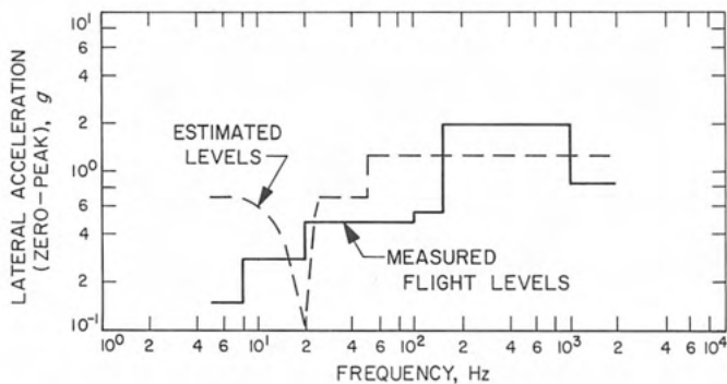
Fig. X-15. Comparison of the 95% flight equivalent sinusoidal vibration environment and the estimated sinusoidal vibration environment for the lateral axes
