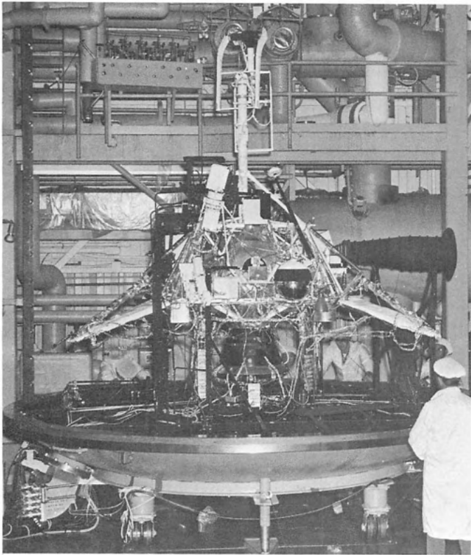
Fig. XI-11. Spacecraft installed on end bell of SERF-C-4S solar simulator
