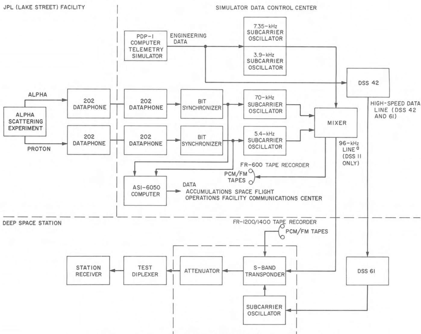
Fig. VII-15. Alpha scattering experiment simulation configuration
