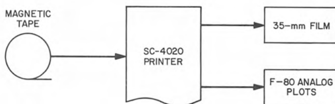
Fig. VII-3. The SFOF peripheral computer equipment input/output
