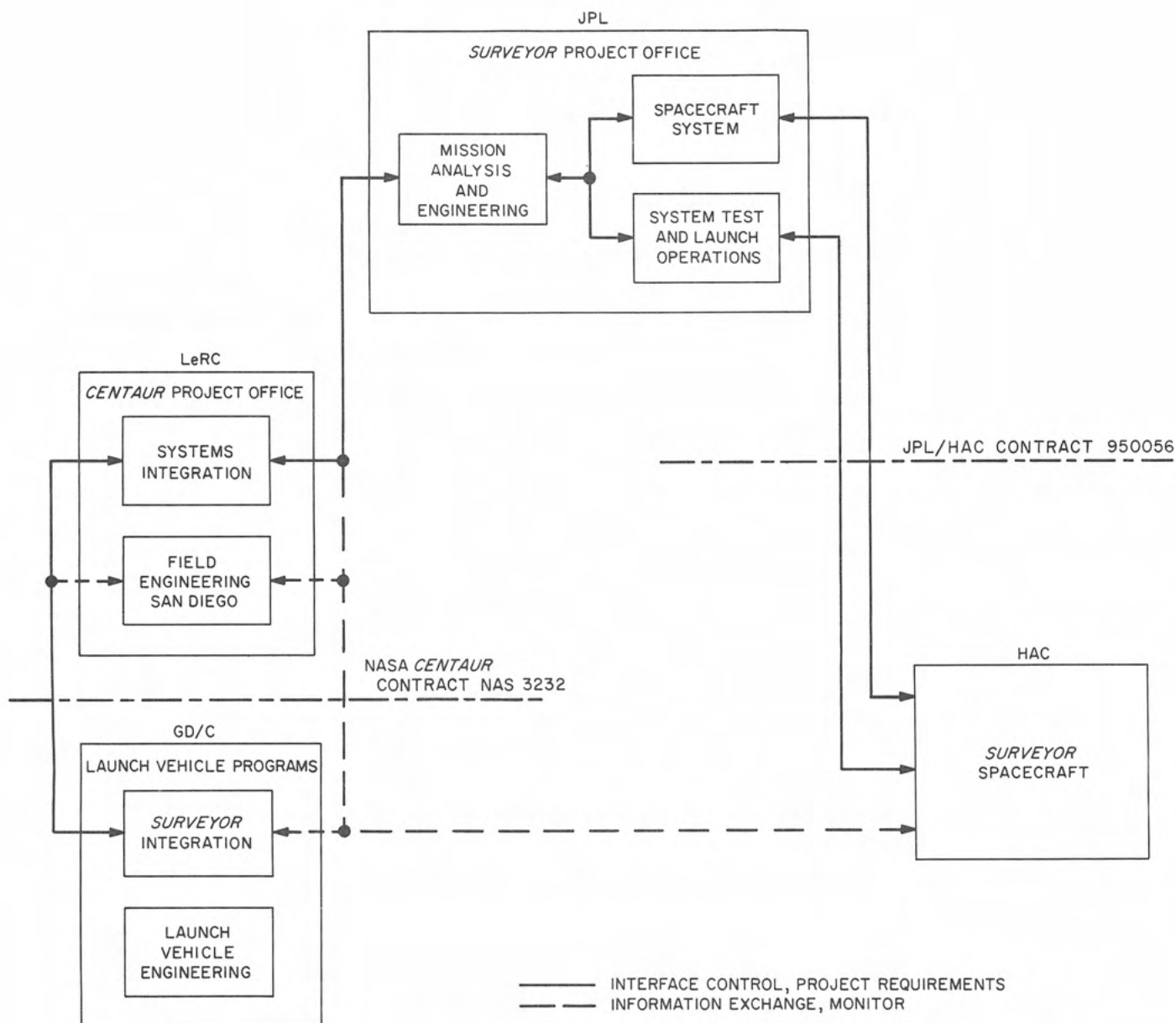
Fig. VIII-4. Spacecraft/Launch Vehicle System interface planning and design operating relationship
