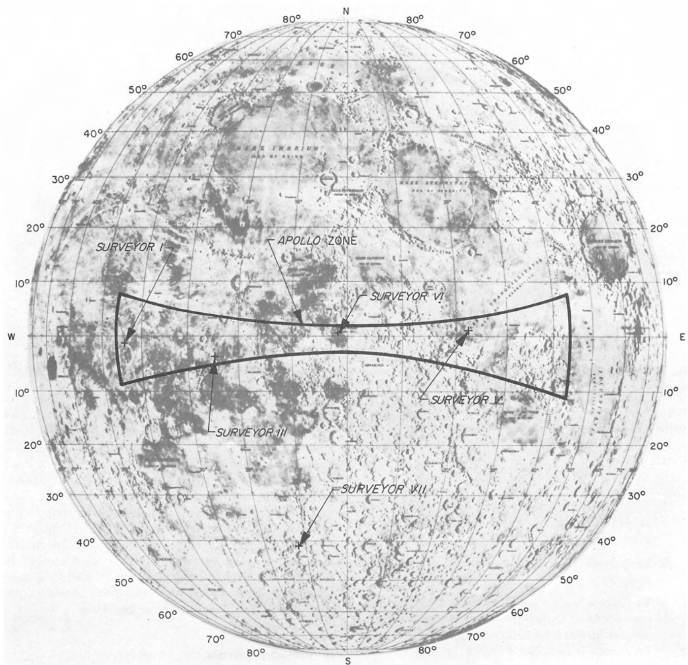
Fig. I-1. Lunar landing sites of Surveyor spacecraft
