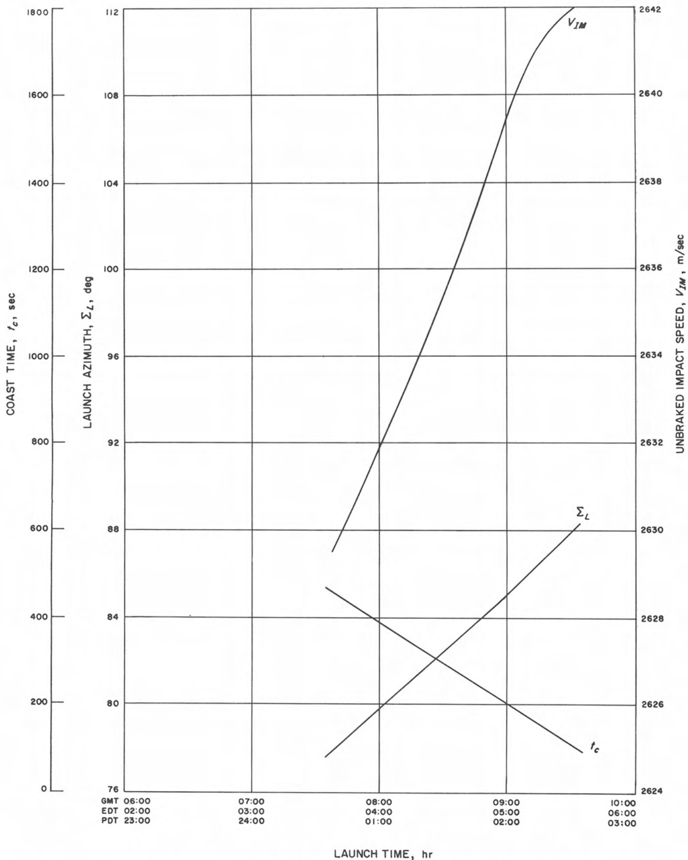
Fig. VI-29. Typical graph of unbraked impact speed, launch azimuth and parking orbit coast time vs launch time
