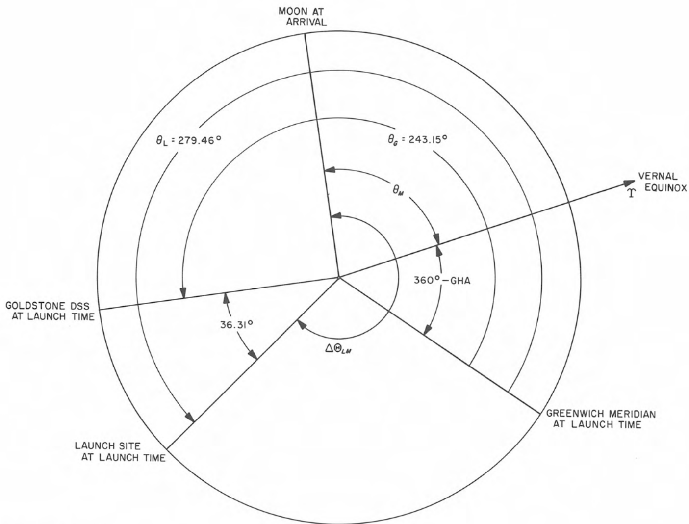
Fig. VI-13. Required excursion in right ascension ( \Delta\Theta_{LM} )
