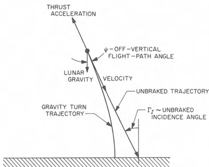
Fig. VI-9. Gravity turn descent geometry
