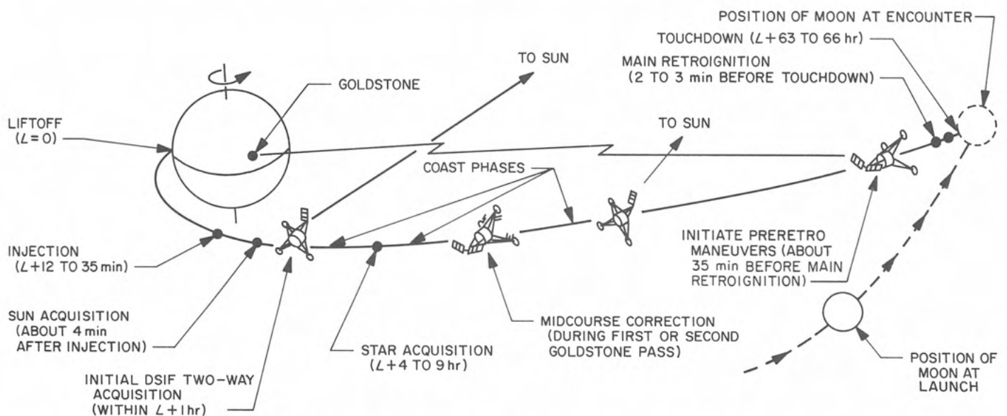
Fig. I-5. Earth-to-moon trajectory—showing major events
