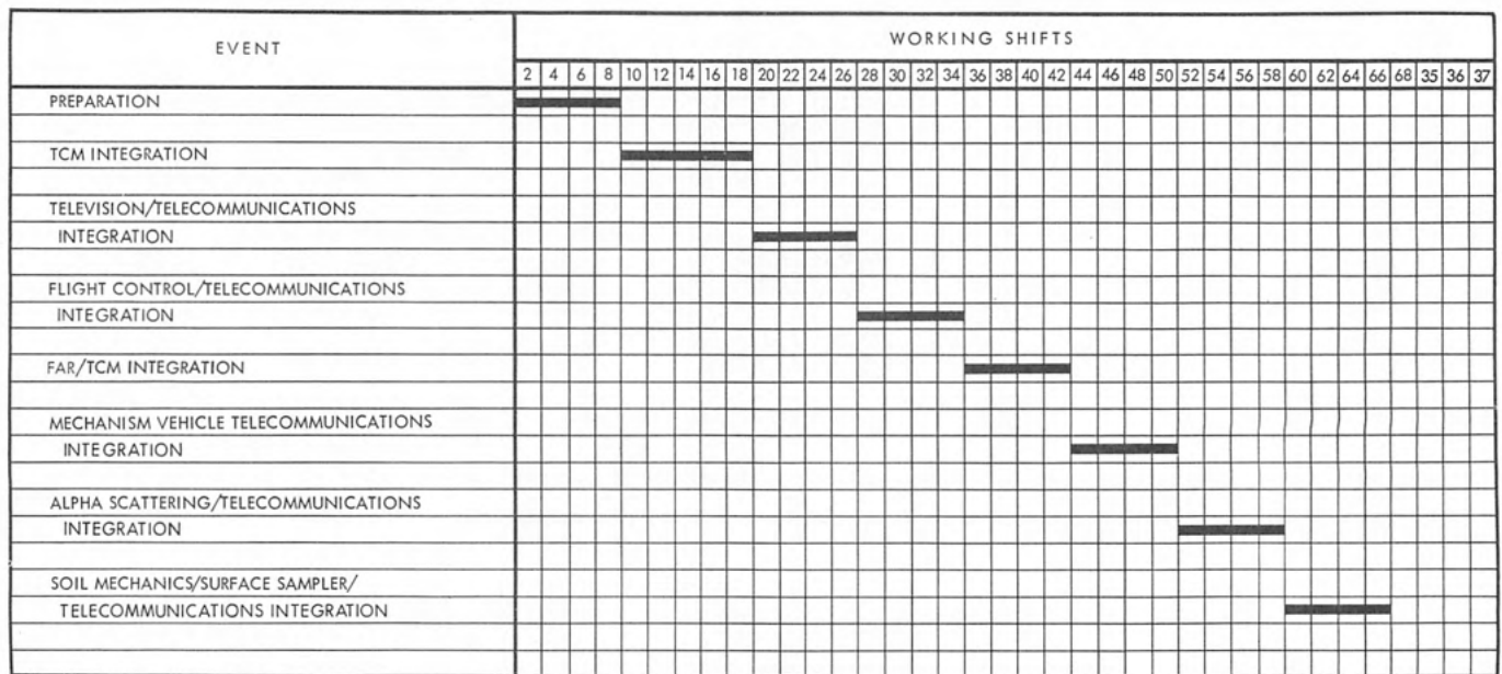
Fig. XI-7. Initial system checkout nominal test schedule
