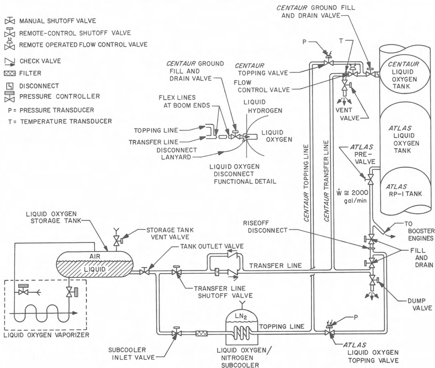
Fig. VIII-27. Liquid oxygen transfer system, Launch Complex 36B
