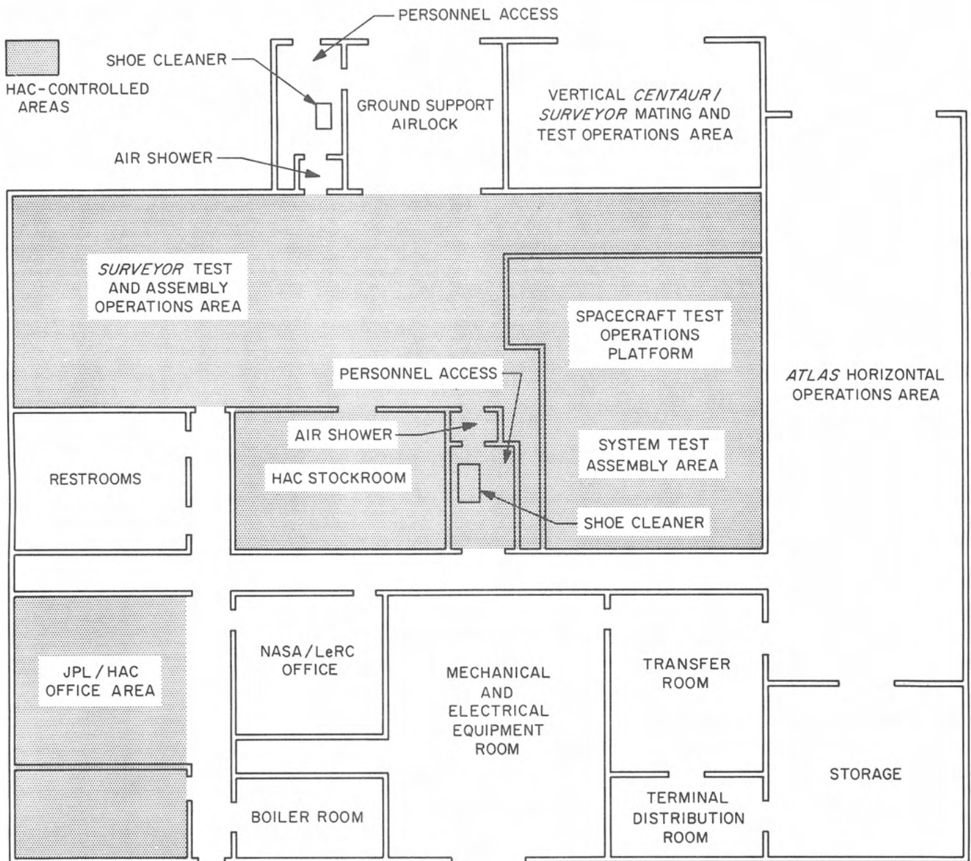
Fig. VIII-21. Combined systems test stand first floor plan
