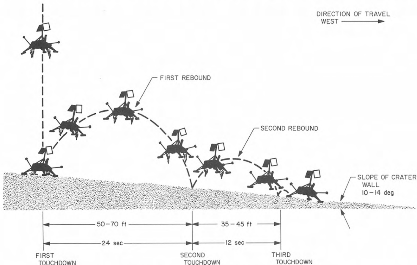
Fig. II-1. Sketch showing events during Surveyor III lunar landing
